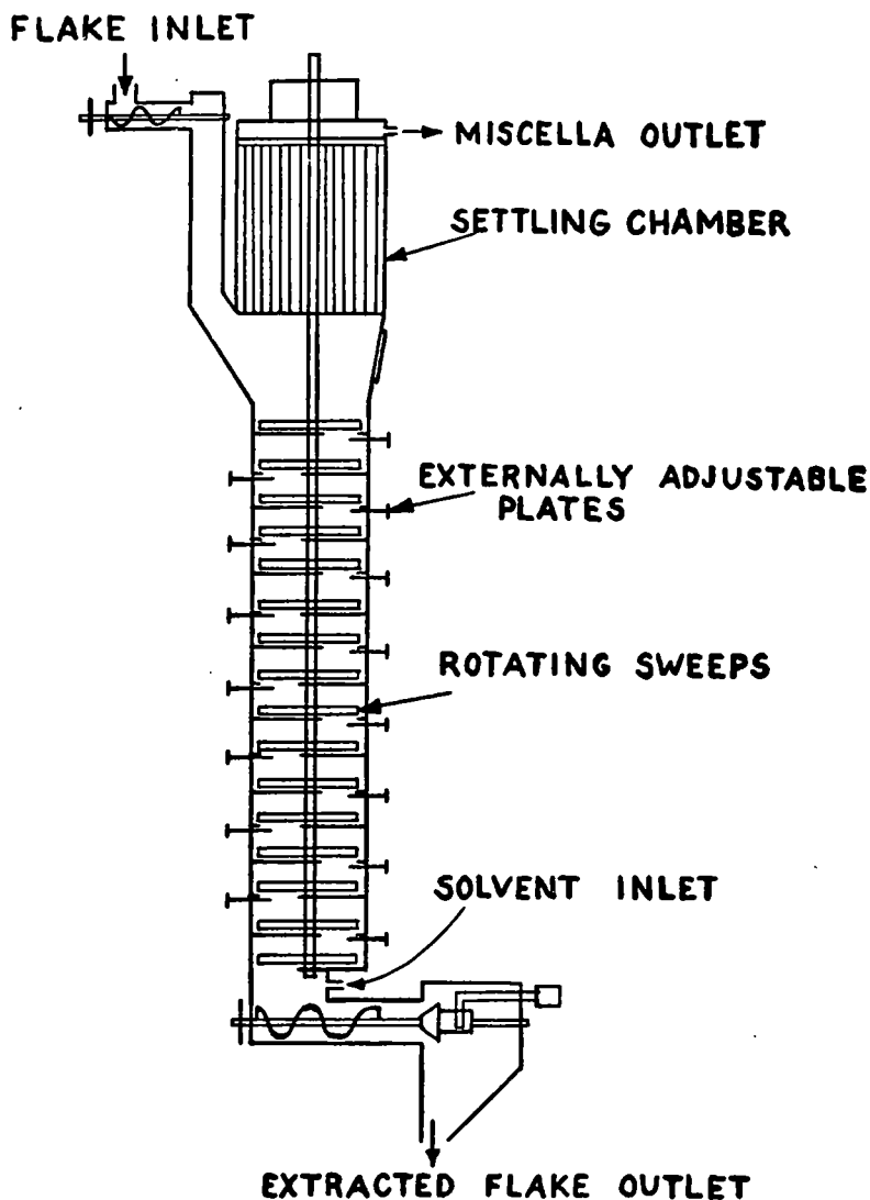
Figure 8. Vertical Total Immersion Extractor.
