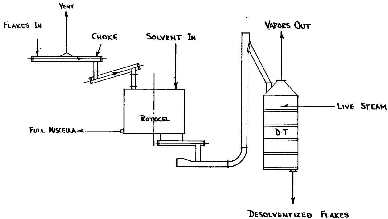
Figure 6. Rotary System.
