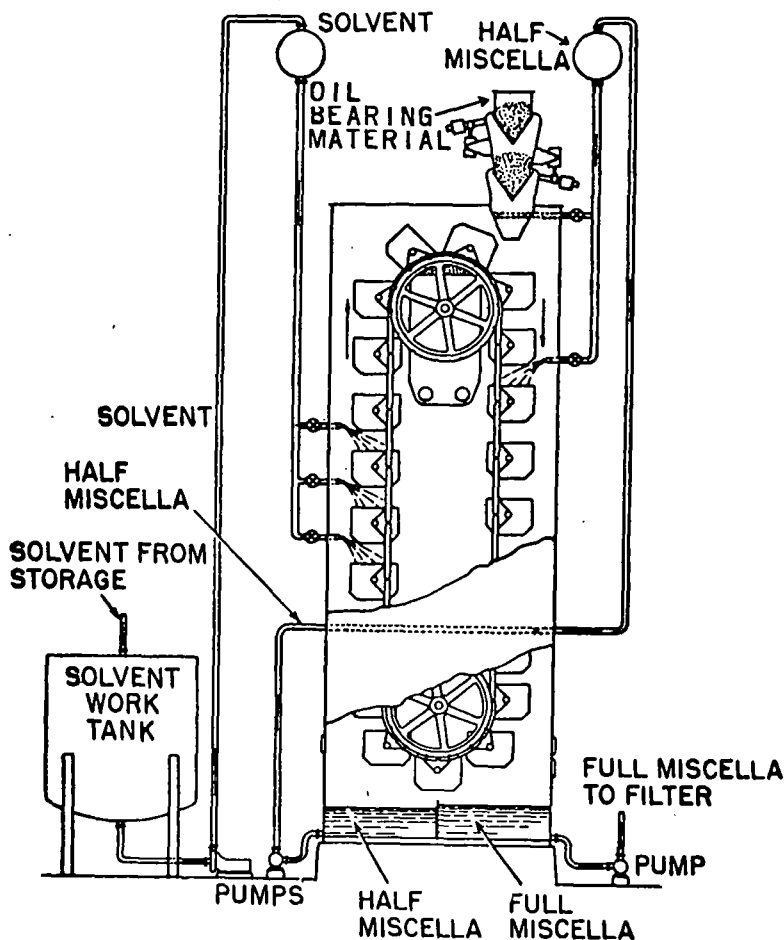
Figure 4. Vertical Basket Extractor.
