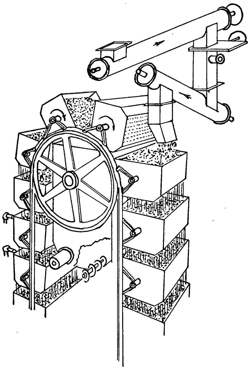
Figure 5. Feeder and Discharge of Basket Extractor.
