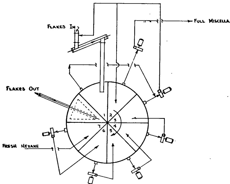
Figure 7. Rotary Extractor.
