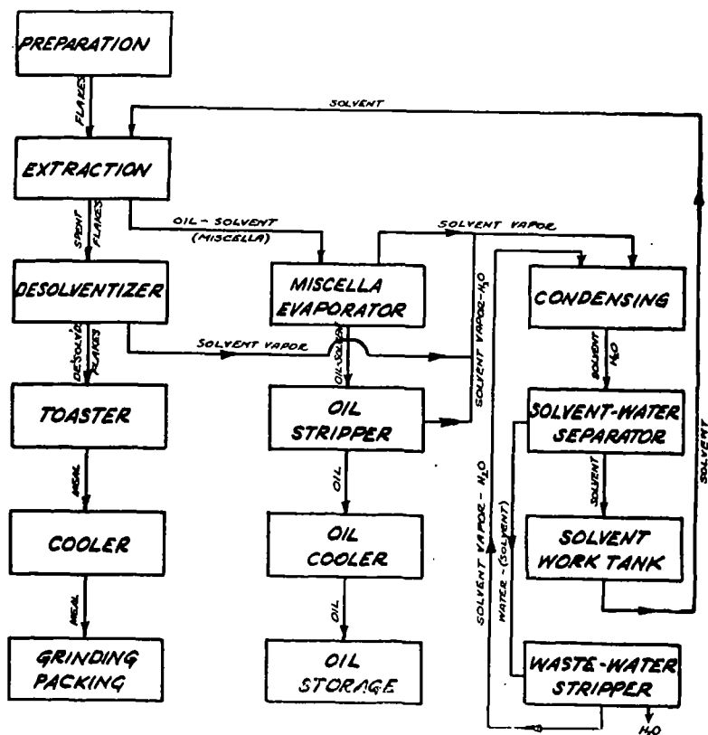
Figure 3. Generalized Flow Diagram.
