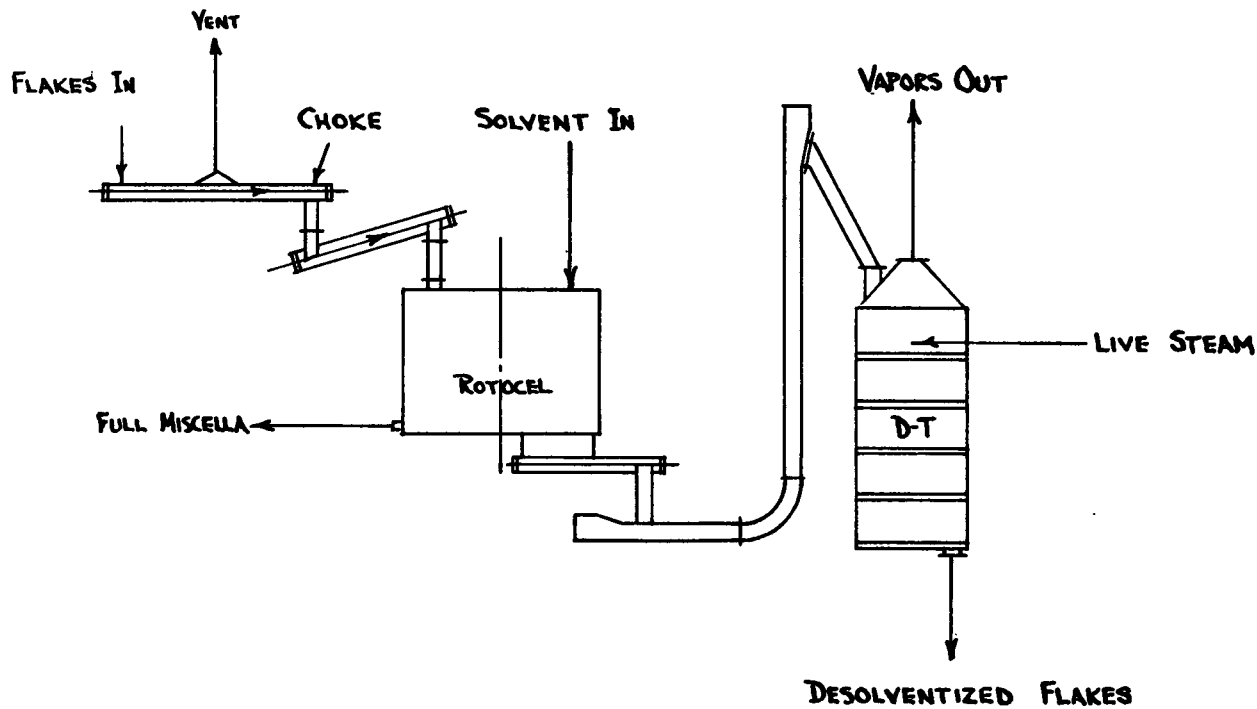
Figure 5. Rotocel System.
