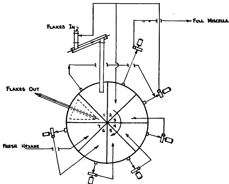
Figure 6. Rotocel Extractor.
