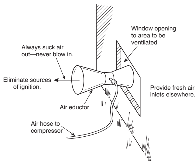
FIGURE 5.4.7.1 Exhaust Ventilation.
