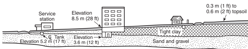
FIGURE C.8.1(b) Effects of Slope of Underground Strata on Groundwater Flow II.
