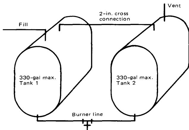
Figure 2-3.2(a) Recommended arrangement of two fuel oil tanks of not more than 660 gal (2500 L) aggregate capacity.
