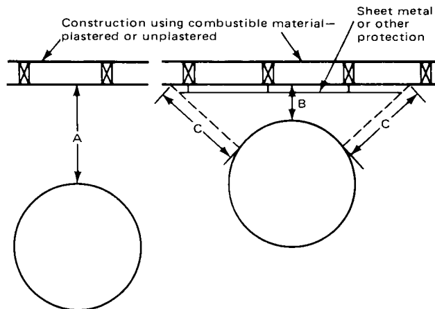
Figure 4-4.1(d) Extent of protection necessary to reduce clearances from appliances or chimney connectors.
