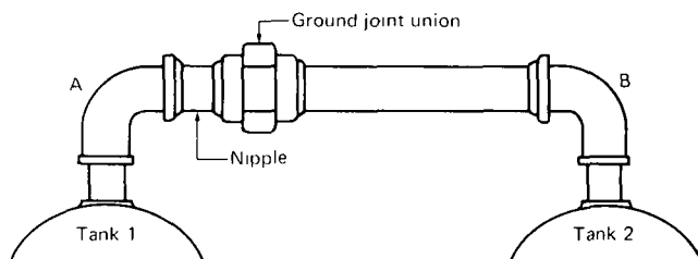
Figure 2-3.2(b) This shows the detail of the cross connection that can be used in Figure 2-3.2(a).
