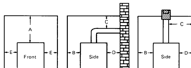
Figure 4-4.1(a) Clearances to combustible materials.
