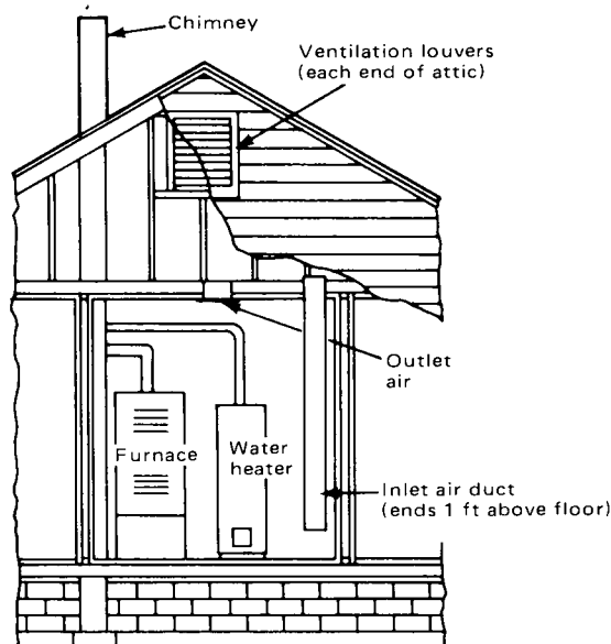
Figure 1-5.4(b) Appliances located in confined spaces — all air from outdoors. (See 1-5.4.2.)
