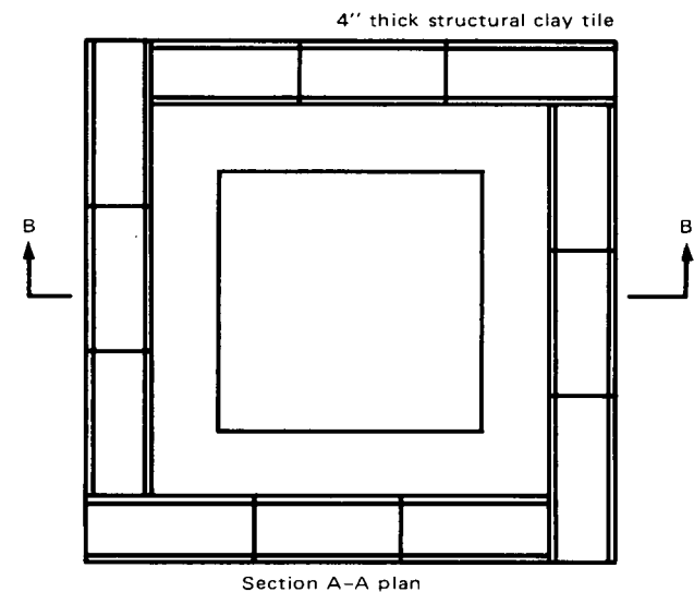
Section A-A plan
