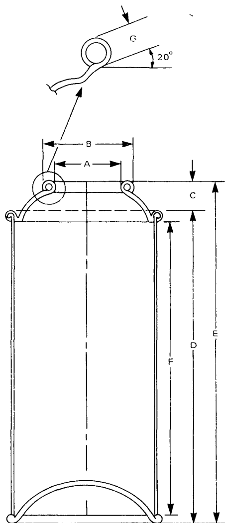
Figure A-1 Typical aerosol container.
