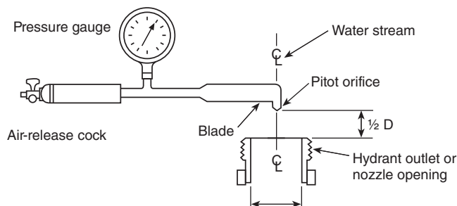
FIGURE 4.8.3 Pitot Tube Position.
