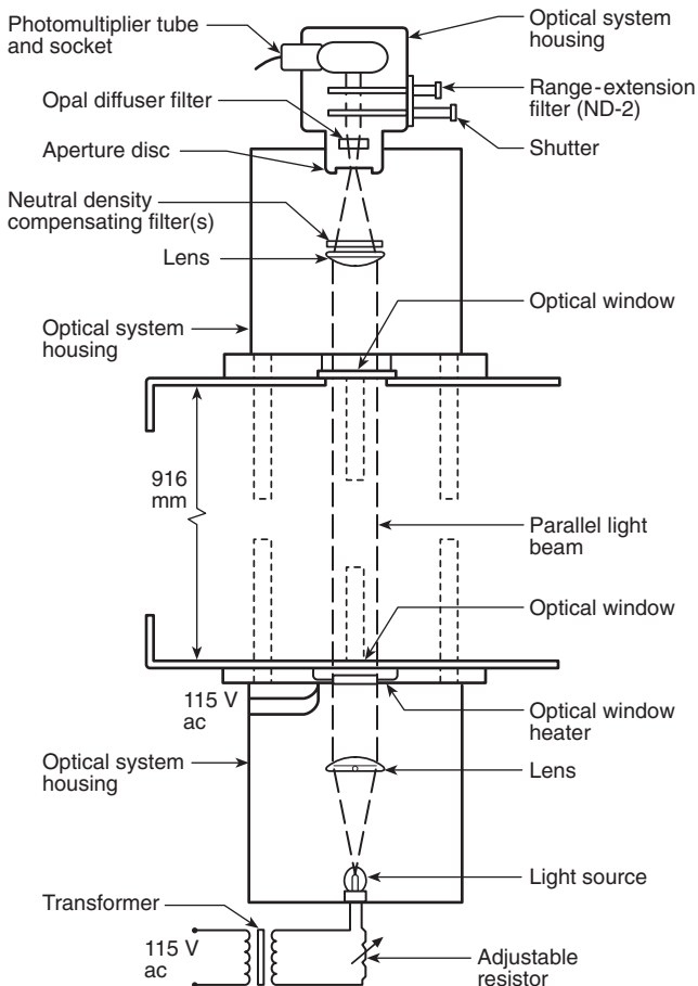
FIGURE 4.5.1.2.1 Photometric System.
