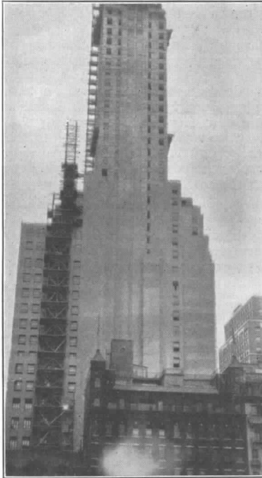
Combustible scaffolding for lower 23 floors; steel scaffolding and flame-proofed planking on upper floors.
