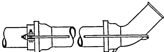
FIG. 96-7. ANCHOR FOR \frac{1}{8} BEND BELL END If distance between joints shown is less than 12 feet, see Note 1.
