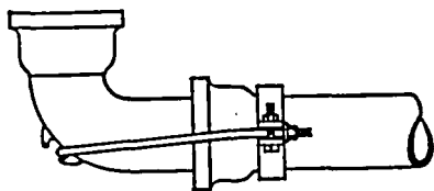
FIG. 96-4. ANCHOR FOR \frac{1}{4} BEND SPIGOT END
