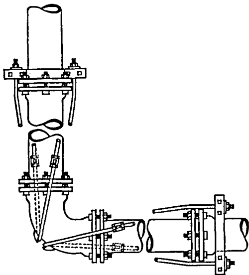
FIG. 96-8. ANCHORS AT \frac{1}{4} BEND
