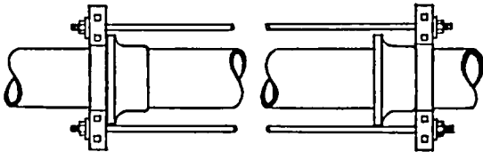
FIG. 96-2. PIPE ANCHOR
