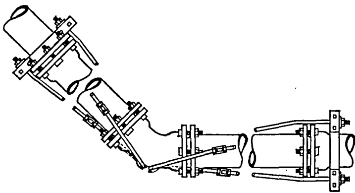
FIG. 96-9. ANCHORS AT \frac{1}{2} BEND
