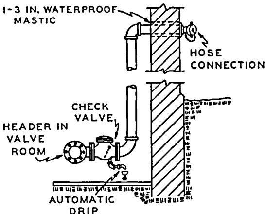
FIG. 26-1. FIRE DEPARTMENT CONNECTION
