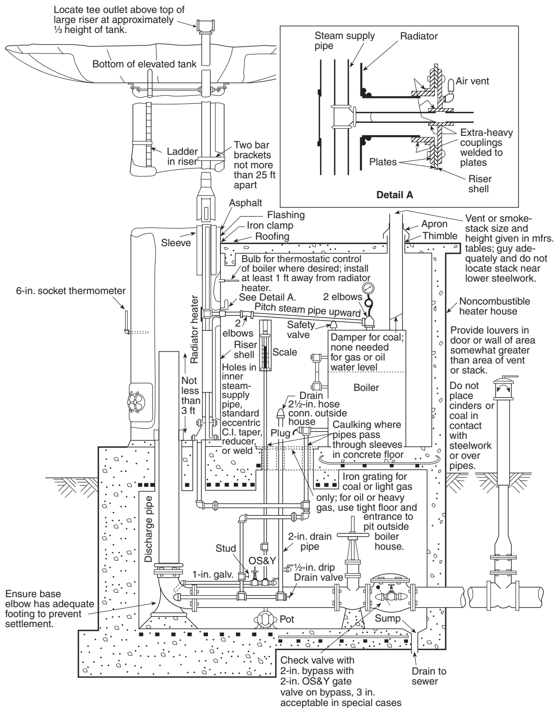
FIGURE 15.3.6.11.1 Aboveground Steam Boiler Radiator Heater Arrangement.
