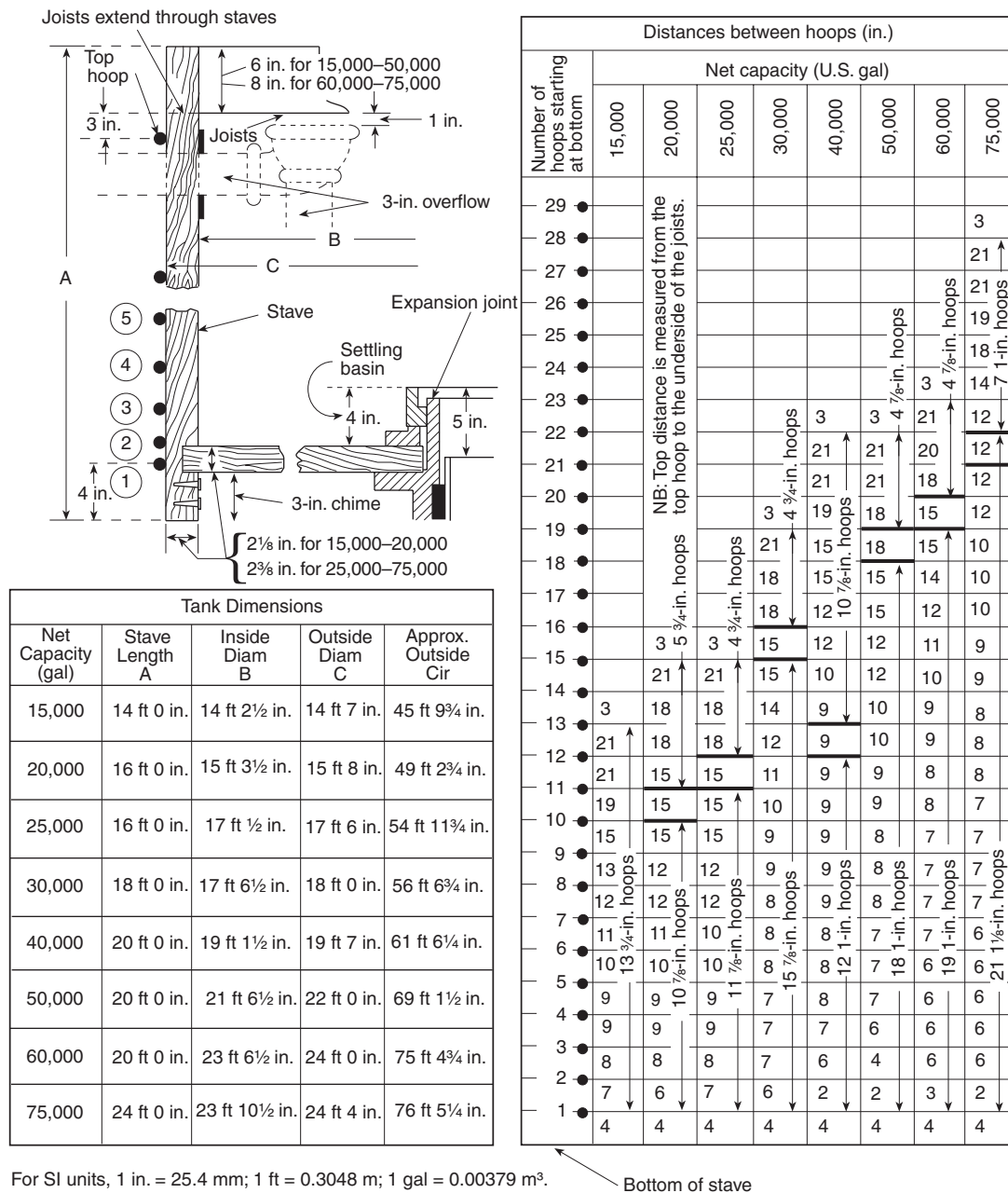
FIGURE A.8.5.3(a) Hoop Schedules for Wood Tanks (dimensions are for cylindrical tanks).
