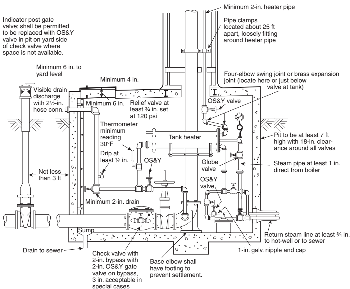
FIGURE 15.1.7.5.5(a) Tank Heater Drain Arrangement at Base of Riser.
