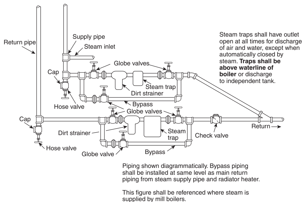
FIGURE 15.3.6.10.3 Steam Trap Arrangement.
