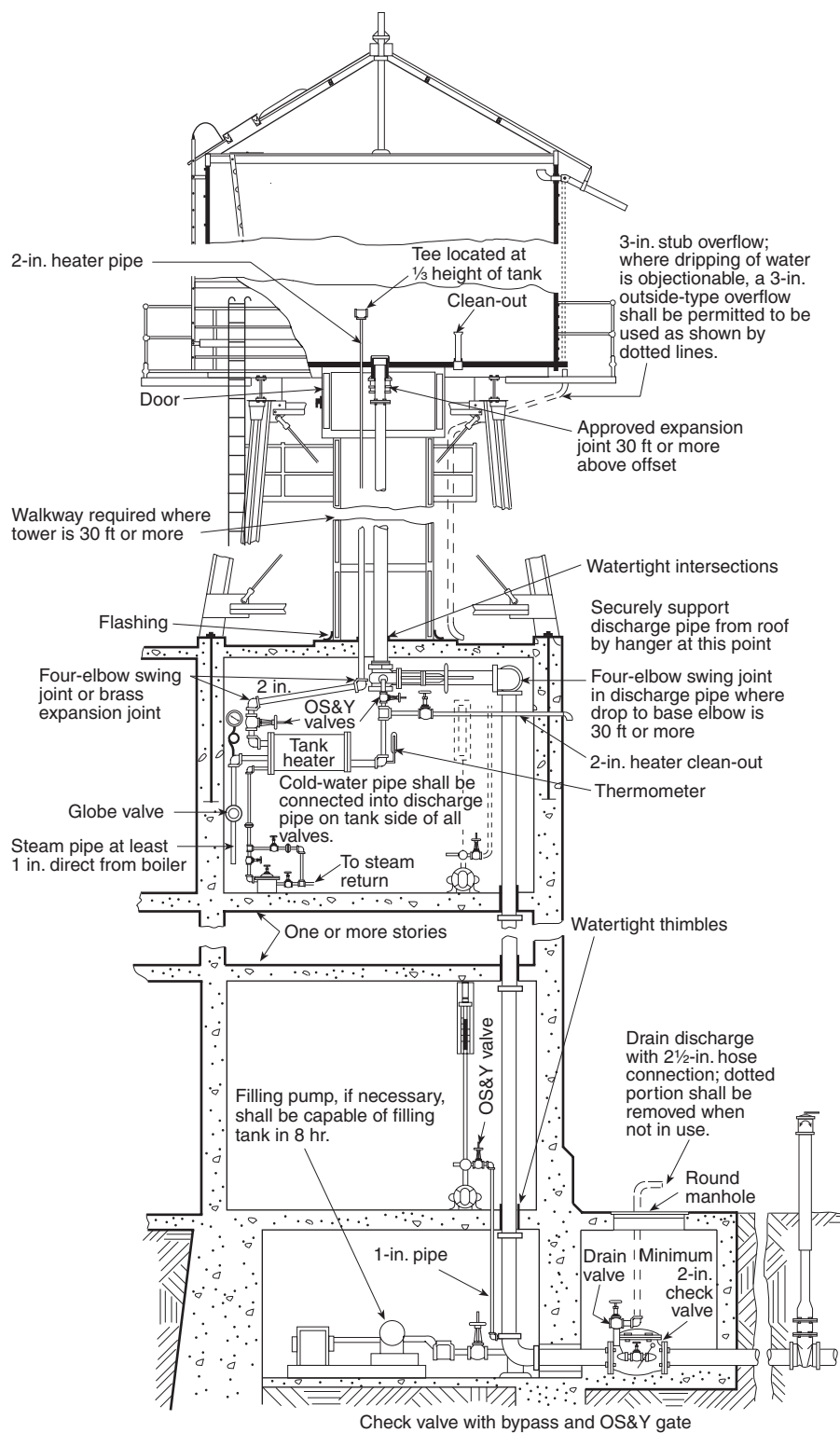
FIGURE 15.1.7.5.5(b) Tank Heater Drain Arrangement.
