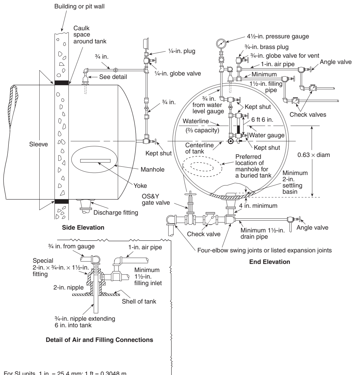
FIGURE B.1(a) Pipe Connections to Pressure Tanks.
