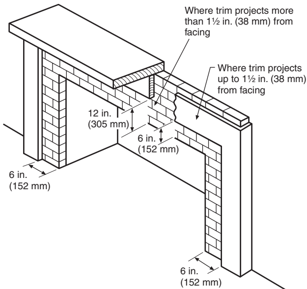
FIGURE 11.2.5.4 Fireplace Clearance to Combustible Material.
