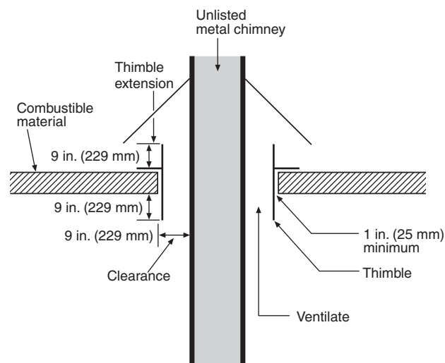
FIGURE 8.2.2.2.7 Ventilating Thimble.
