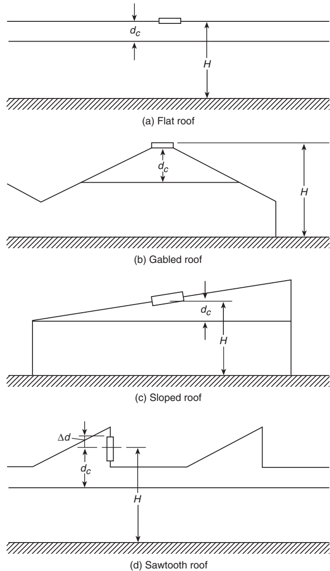
FIGURE 5.4.2 Measurement of Ceiling Height ( H ) and Curtain Board Depth ( d_c ).
