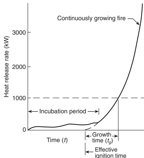
FIGURE 8.3.1 Conceptual Illustration of Continuous-Growth Fire.
