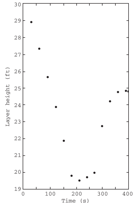
FIGURE C.7(a) Plot of the Height of the Smoke Layer Interface vs. Time for the Default Simulation.
