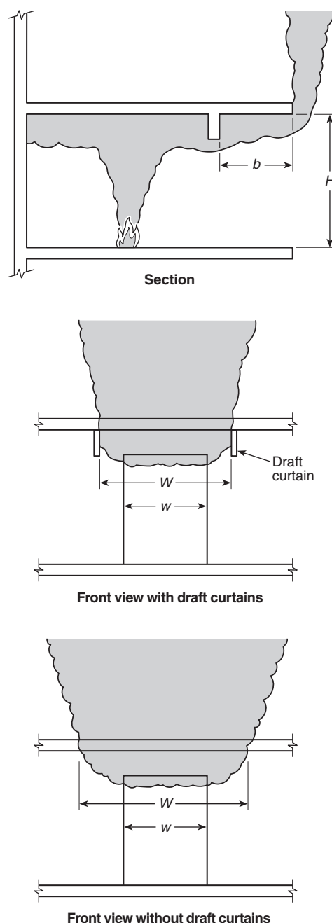
FIGURE A.3.3.3 Smoke Layer.
