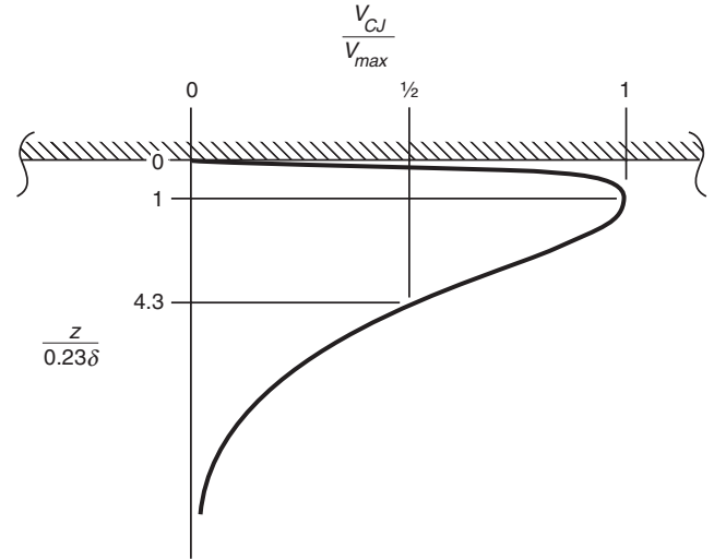
FIGURE B.5.2 A Plot of Dimensionless Ceiling Jet Velocity Distribution, V_{CJ}/V_{max} , as a Function of z/0.23\delta per Equation B.52.
