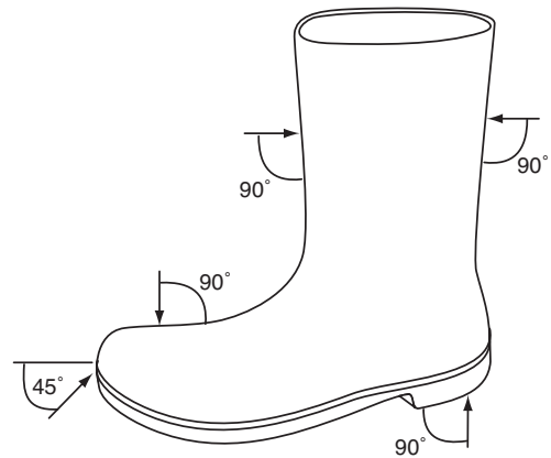
FIGURE 8.32.5.2 Test Areas.
