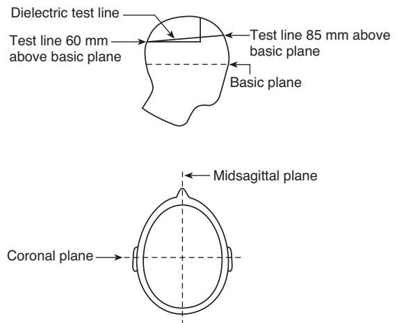
FIGURE 8.21.5.1.2 Test Setup.
