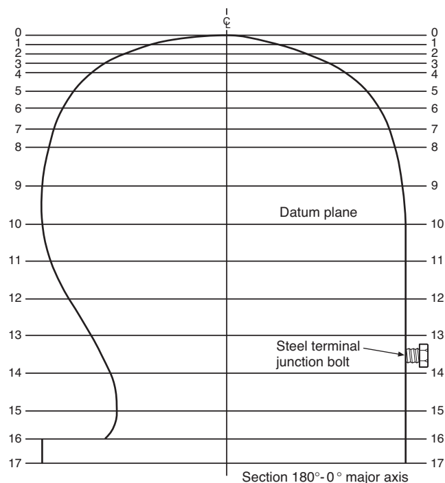
FIGURE 8.19.4.1(b) ISEA Size 7 Headform, Side with Modification for Steel Terminal Junction Bolt.
