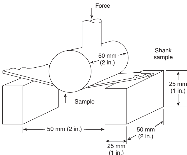
FIGURE 8.34.4 Shank Bend Test Setup.
