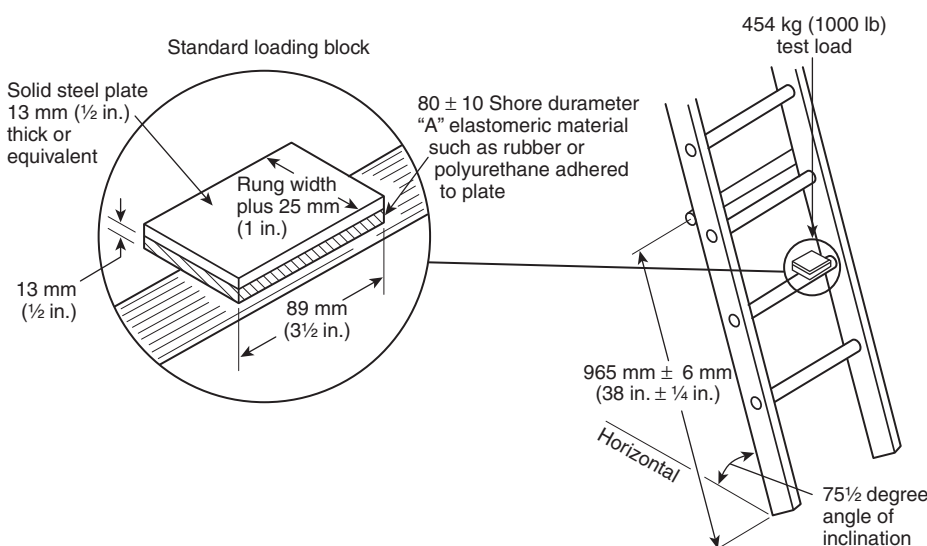
FIGURE 6.2.4.1.1 Design Verification Rung-to-Beam Shear Strength Test.
