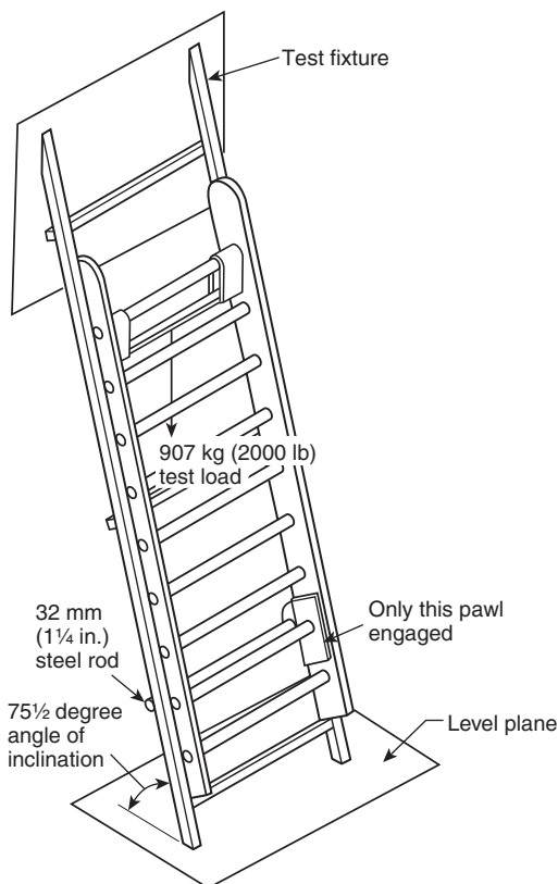
▲ FIGURE 6.4.2.2 Design Verification Single Pawl Load Test.
