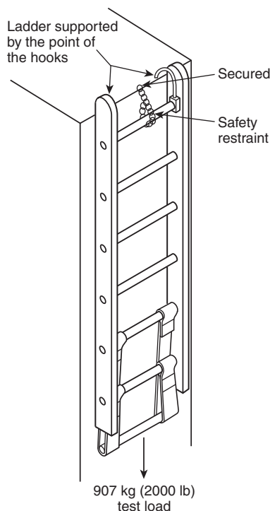
FIGURE 6.3.1 Design Verification Roof Hook Test.
