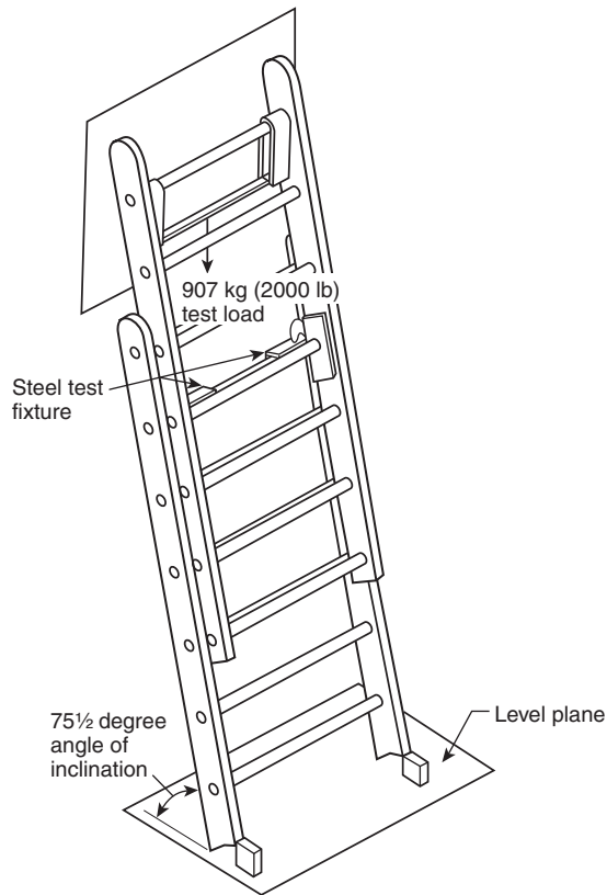
▲ FIGURE 6.4.3.2 Design Verification Pawl Tip Load Test.
