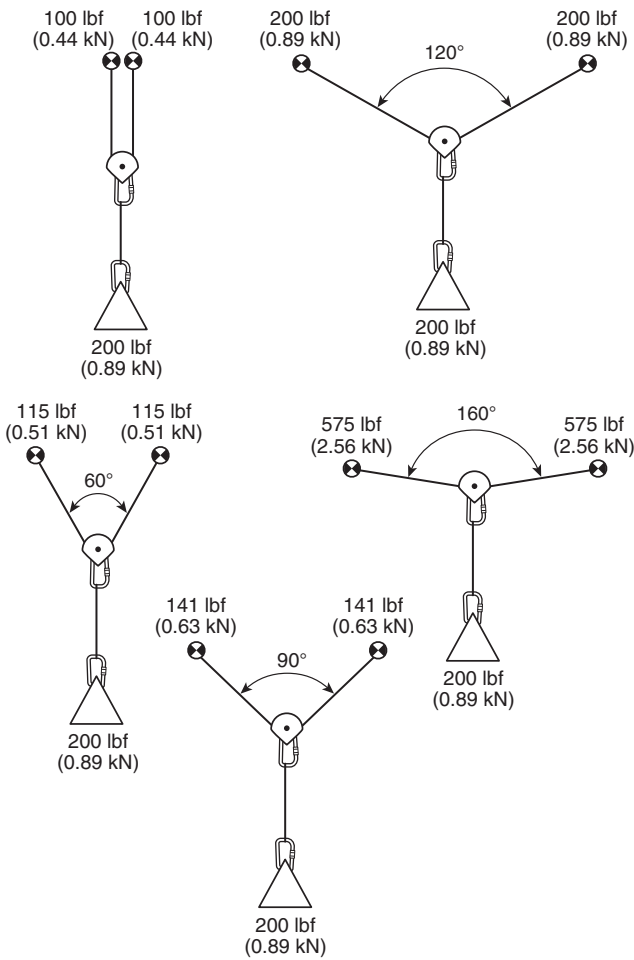
FIGURE A.3.3.27 Two-Point Anchor Systems Showing Relative Force.
