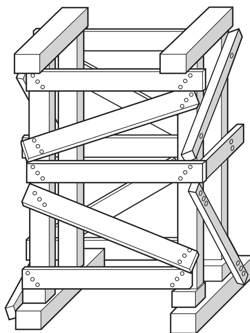
FIGURE A.6.4.3(6)(a) Laced Post Shore.
