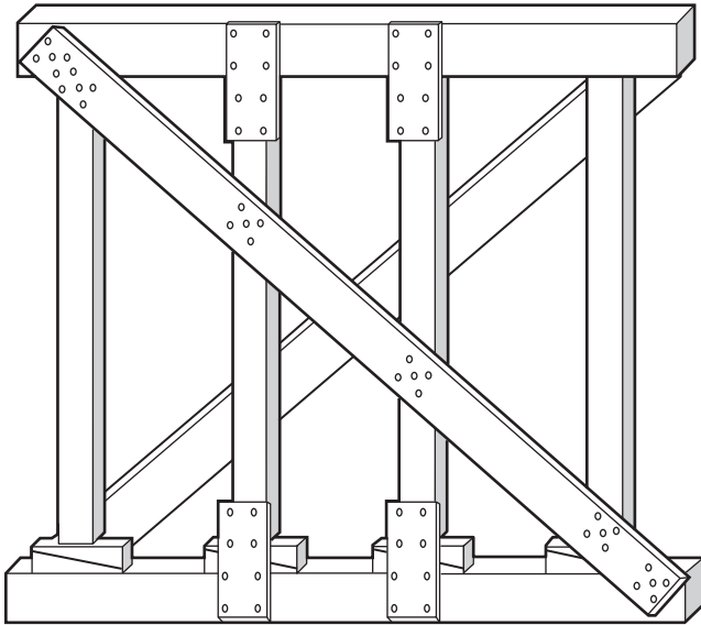
FIGURE A.6.3.3(6)(d) Multi-Post Vertical Shore.
