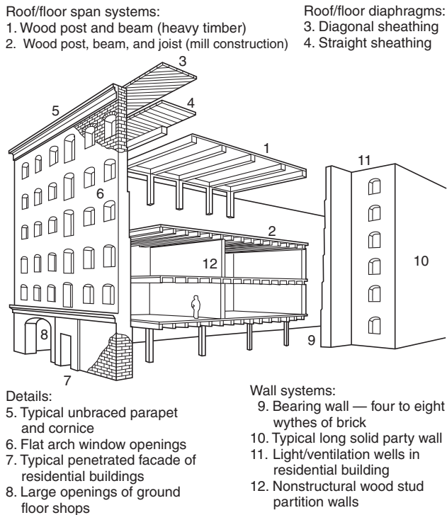
FIGURE C.1(n) Unreinforced Masonry Bearing Wall, Example 3 of 3.
