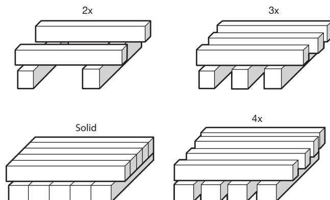
FIGURE A.6.3.3(6)(j) Box Cribbing.
