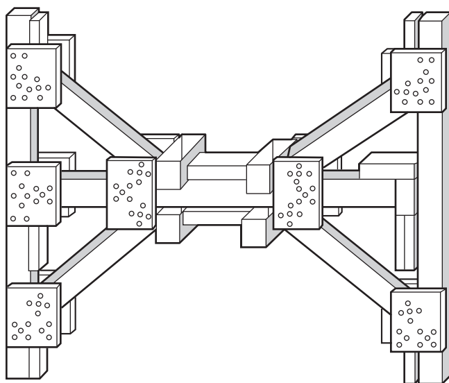
FIGURE A.6.4.3(6)(f) Flying Shore.
