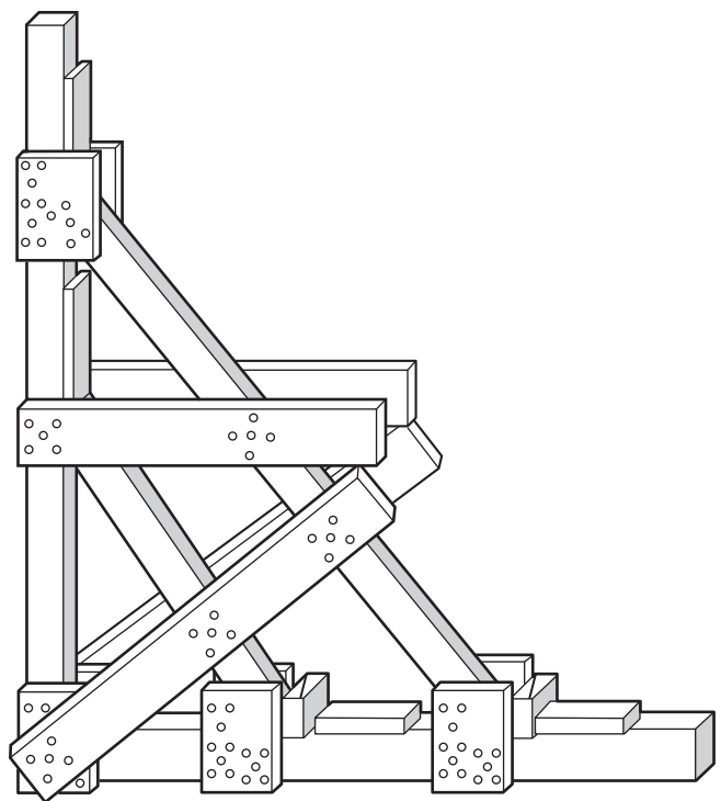
FIGURE A.6.4.3(6)(e) Double Raker Shore.
