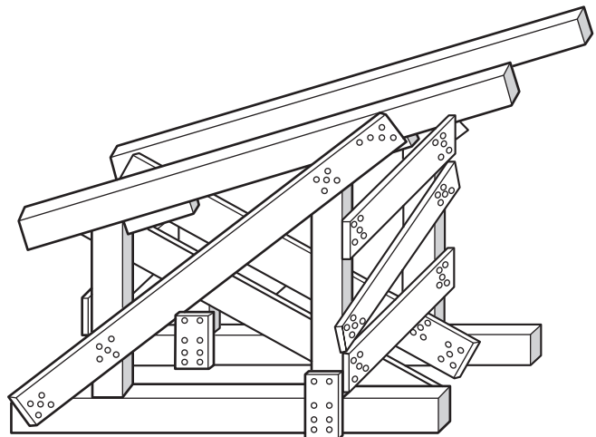
FIGURE A.6.4.3(6)(d) Sloped Floor Shore Type 3.
