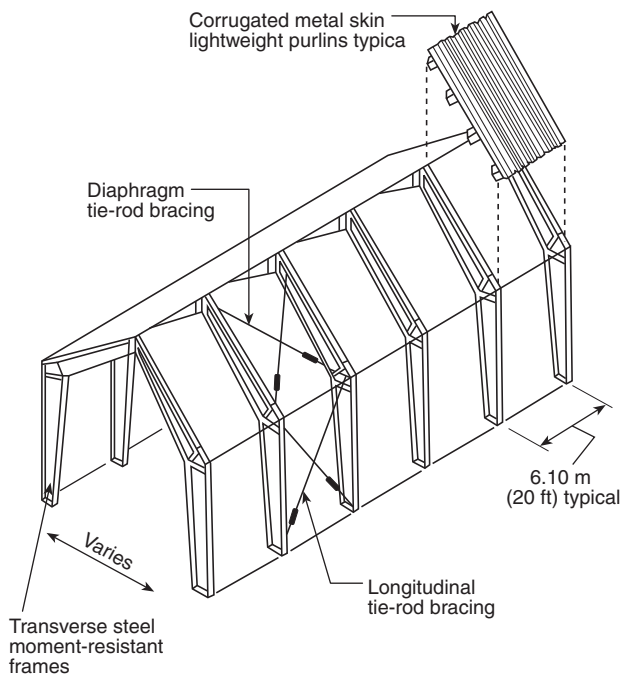
FIGURE C.1(e) Light Metal Construction.
