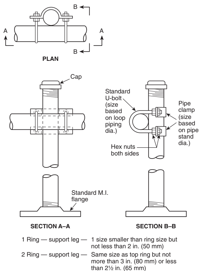
FIGURE A.6.3.2.8(b) Acceptable Attachment for Pipe to Support Legs — Example 1.
