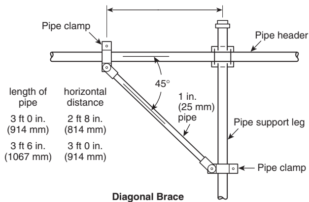
Diagonal Brace
