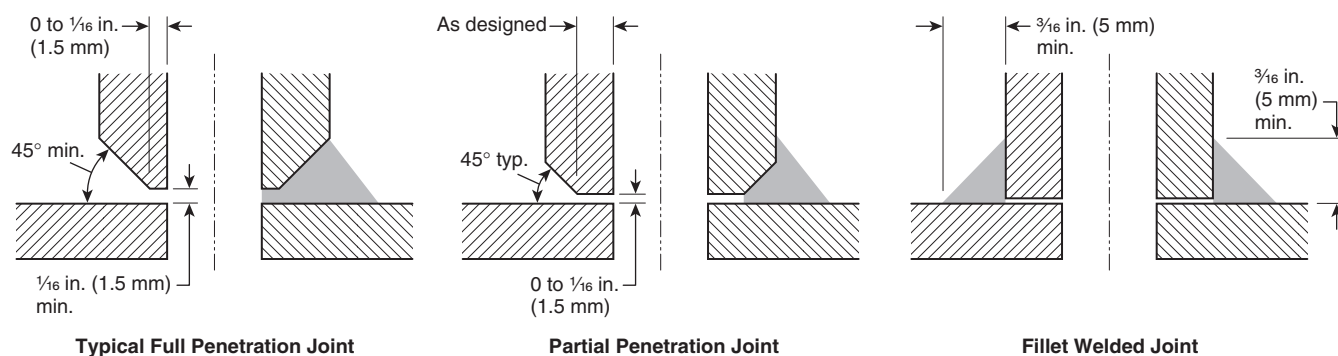
FIGURE A.5.5.2.4.1 Acceptable Joint Configurations for Welding Outlets.
