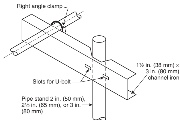
FIGURE A.6.3.2.2.7 Support Leg Footings.
