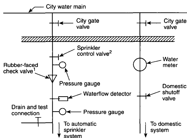
Figure A-2-3.2(a) Preferable arrangement.
