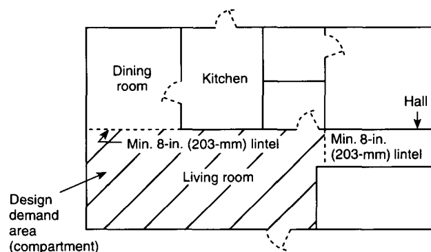
Figure A-2-5.1.2(b) Sprinkler design areas for typical residential occupancy.
