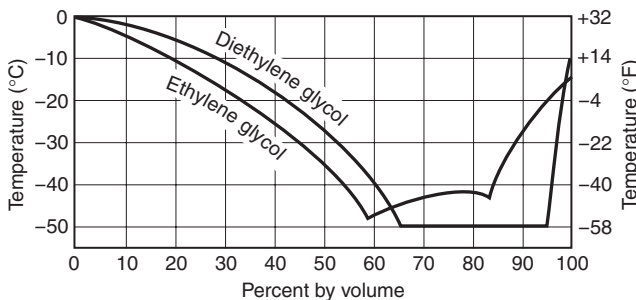
FIGURE A.8.3.2.6 Freezing Points of Water Solutions of Ethylene Glycol and Diethylene Glycol.
