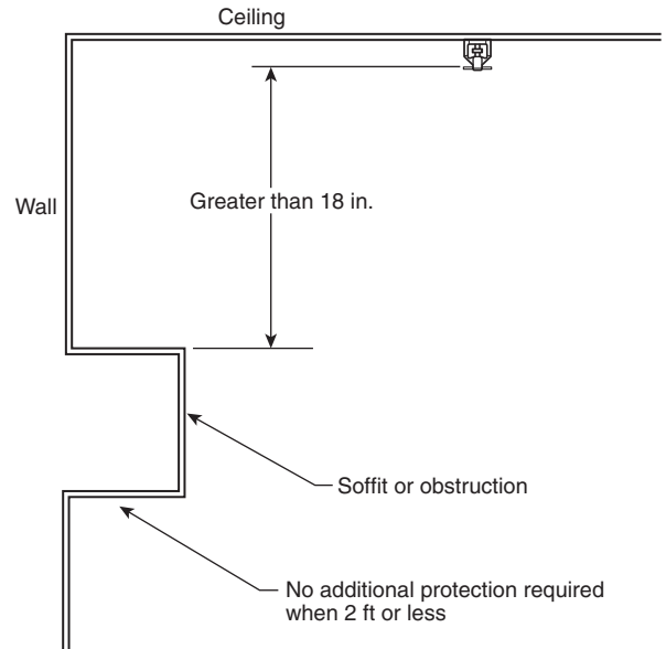
FIGURE A.8.8.5.1.2 Soffit/Obstruction Against Wall Greater Than 18 in. (457 mm) Below Deflector.
