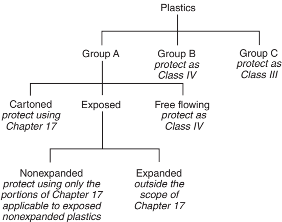
FIGURE 17.1.2.1 Decision Tree.
