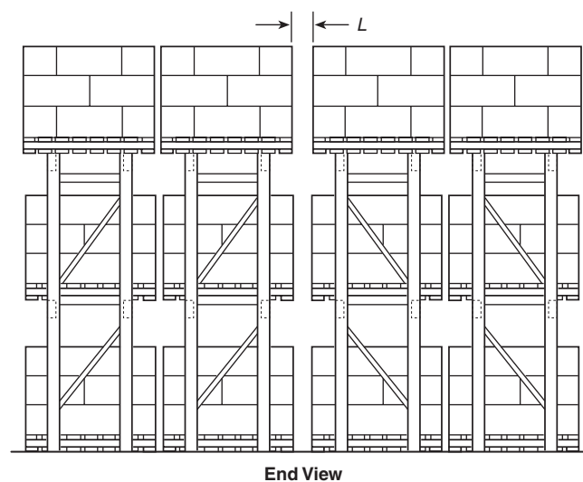
FIGURE A.3.9.3.7(f) Multiple-Row Rack Served by Reach Truck.
