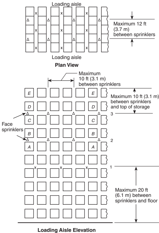
FIGURE 16.3.1.3.1.3(A)(a) In-Rack Sprinkler Arrangement, Class I Commodities, Multiple-Row Racks, Storage Height Over 25 ft (7.6 m).
