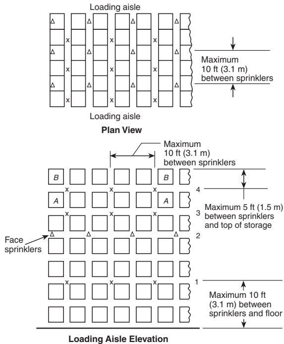
FIGURE 16.3.1.3.1.3(A)(c) In-Rack Sprinkler Arrangement, Class I, II, III, or IV Commodities, Multiple-Row Racks, Storage Height Over 25 ft (7.6 m).
