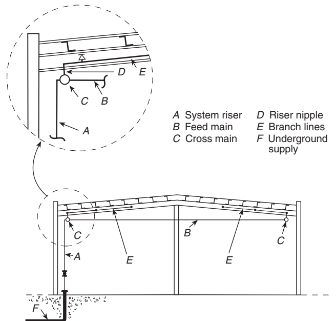
FIGURE A.3.5 Building Elevation Showing Parts of Sprinkler Piping System.
