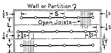
Sprinklers on Alternate Lines Staggered
