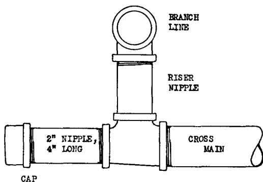
Fig. 435. Flushing Connection.
