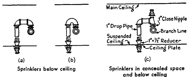
Fig. 419. Pendent Sprinklers at Suspended Ceiling.
