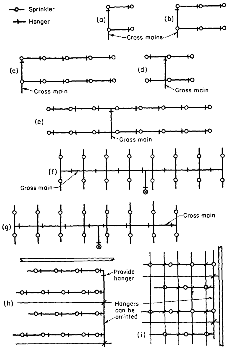
Fig. 533. Location of Hangers. (Not to scale.)
