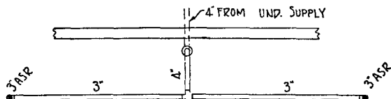
Two 3-inch risers.
