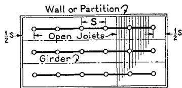
Sprinklers on Alternate Lines Unstaggered
