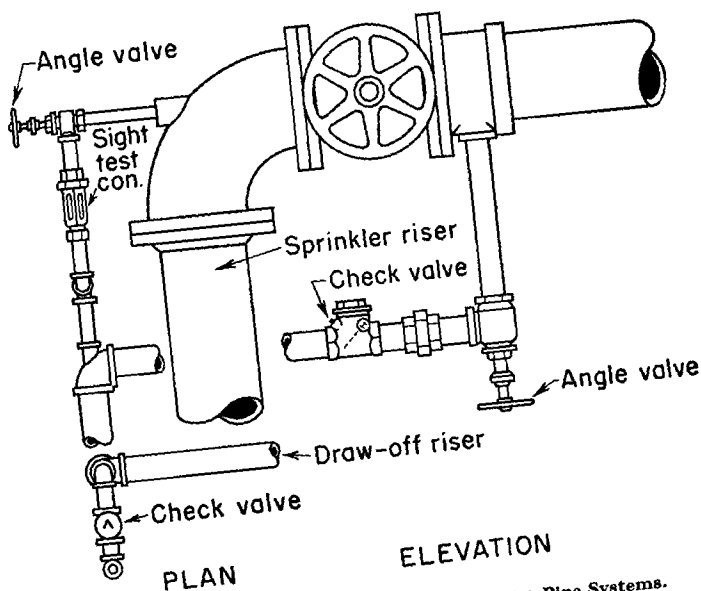
Fig. 451. One-inch System Test Pipes on Wet-Pipe Systems. Connect to top of main riser or to sprinkler main in the highest part of system, which main must be at least 1 in. in size.
