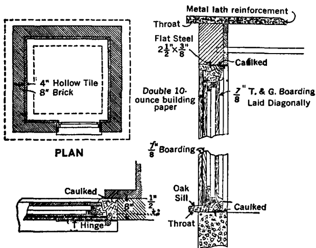
Fig. 843-1. Dry-Pipe Valve Enclosures — Fire-Resistive Construction, Located Outside of Building with no Direct Communication to Building.
