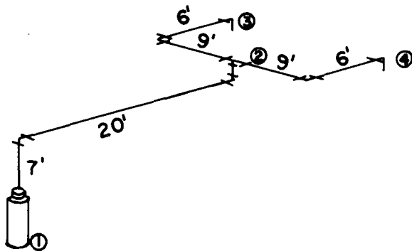
Figure A-1-10.6.5 Calculated Solution.
