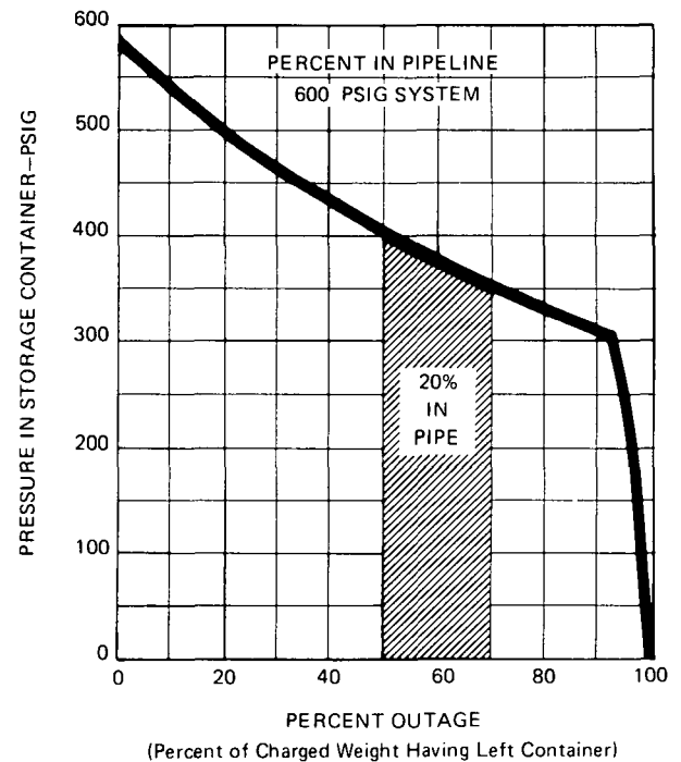
Figure A-1-10.6.3(c) Percent Outage.
