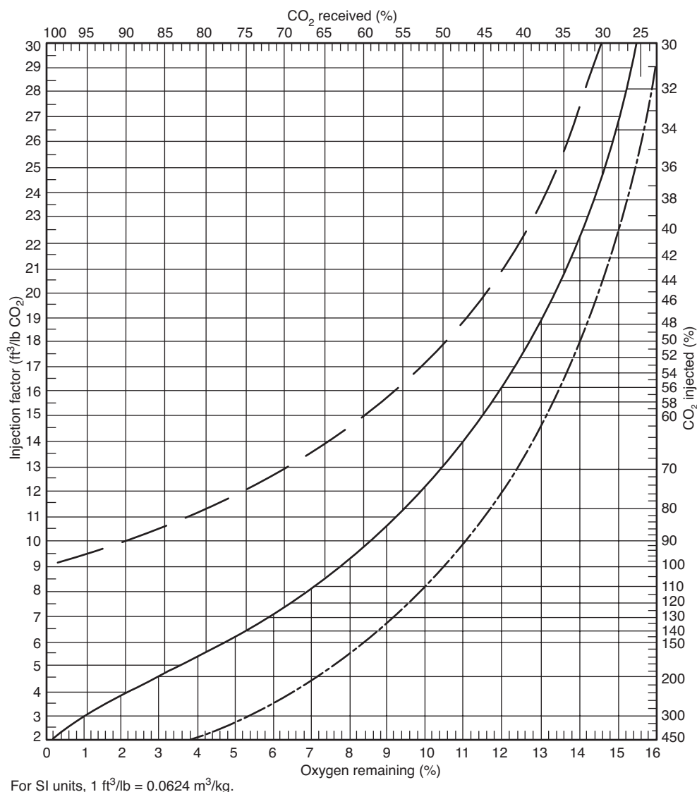
FIGURE D.1(a) Carbon Dioxide Requirements for Inert Atmospheres [based on a carbon dioxide expansion of 9 ft 3 /lb (0.56 m 3 /kg)].
