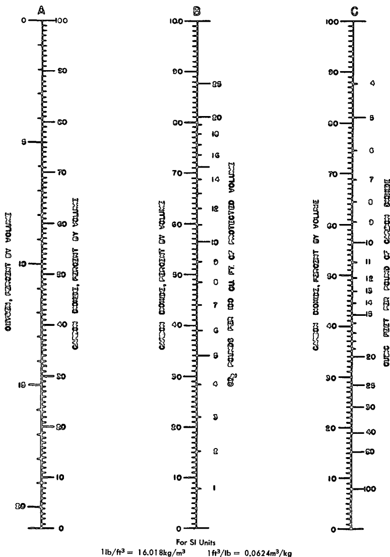
Figure A-2-1(B) Carbon dioxide requirement for inert atmospheres (based on a carbon dioxide expansion of 8.35 cubic feet per pound [0.52 \text{m}^3/\text{kg} ]). Column A shows oxygen content of air-carbon dioxide mixtures; column B shows weight of carbon dioxide in air-carbon dioxide mixtures; column C shows cubic feet per pound of carbon dioxide in air-carbon dioxide mixtures.
