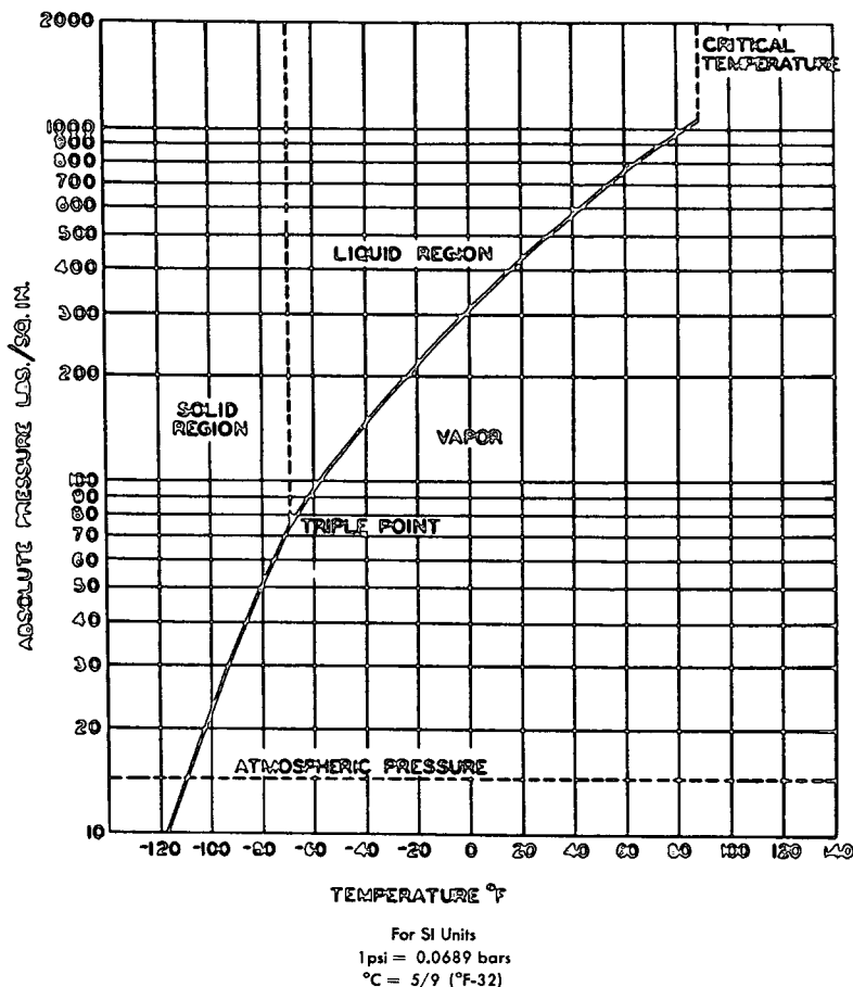
Figure A-1-5.2 Variation of pressure of carbon dioxide with change in temperature (constant volume). Below the critical temperature (87.8°F [31°C]), carbon dioxide in a closed container is part liquid and part gas. Above the critical temperature it is entirely gas.
