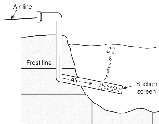
FIGURE A.8.4.6(c) Air Injection Frost-Proofing System.
