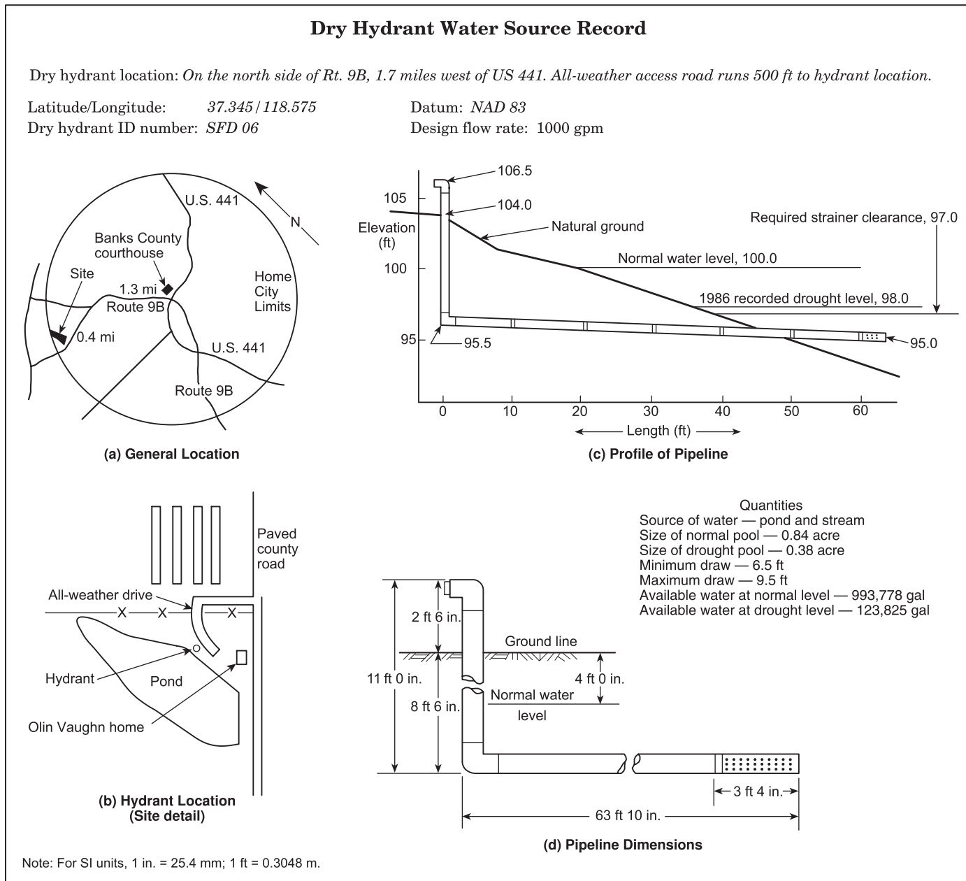
▲ FIGURE A.8.8(a) Example of Dry Hydrant Water Source Record.
