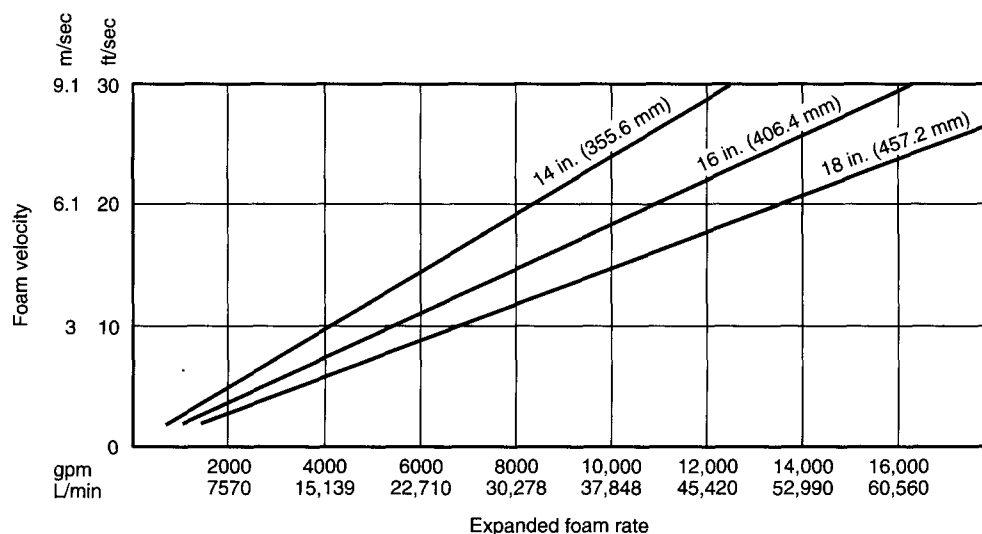
Figure A-3-2.4.2(b) Foam velocity vs. pipe size (14 in., 16 in., and 18 in.) — standard schedule 40 pipe.
