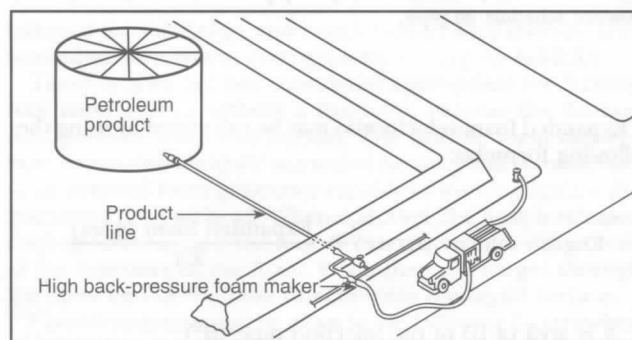
Figure A-3-2.4.1(a) Semifixed subsurface foam installation.
