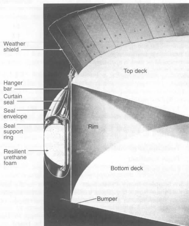
Figure 3-3(b) Tube seal open-top floating roof tank.
