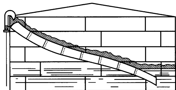
Figure A-1-4(o) Foam trough.
