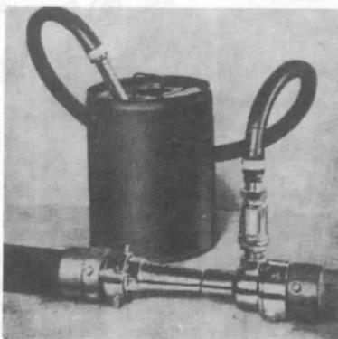
Figure A-1-4(g) In-line eductor.
