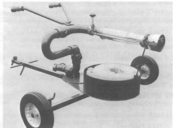
Figure A-1-4(e) Wheeled portable foam-water monitor.
