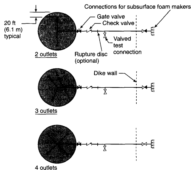
Figure A-3-2.4.2(d) Typical arrangement of semifixed subsurface system.
