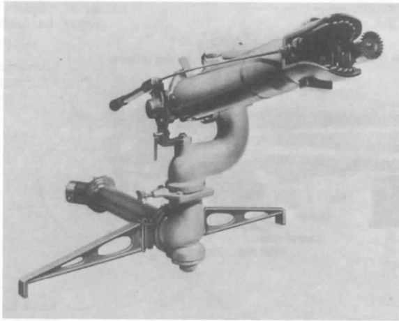
Figure A-1-4(f) Portable foam-water monitor.
