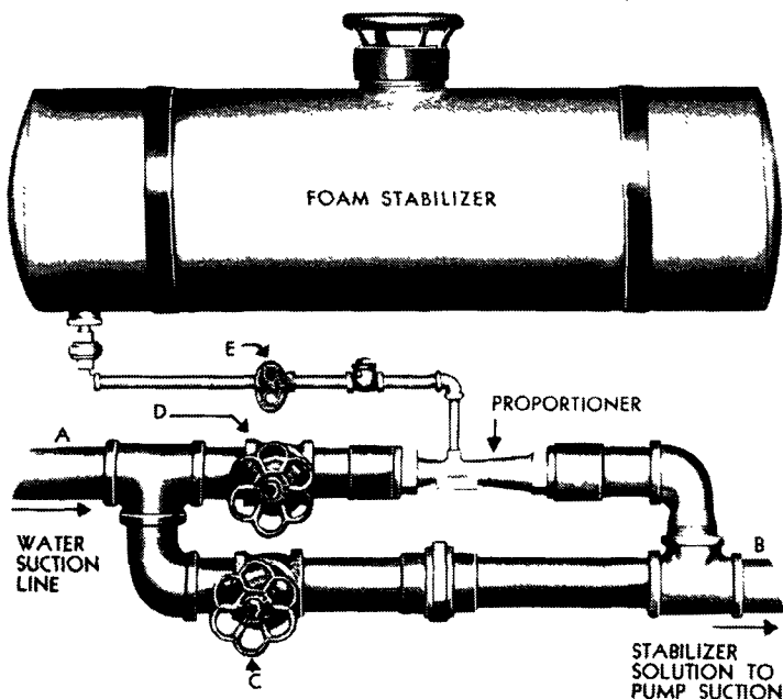
Fig. A-1157(b) (1). Pump Suction Proportioner. To install: connect A to water suction line, connect B to suction side of pump. To operate foam system: close valve C, open valves D and E. To discharge plain water: close valves D and E, open valve C.
