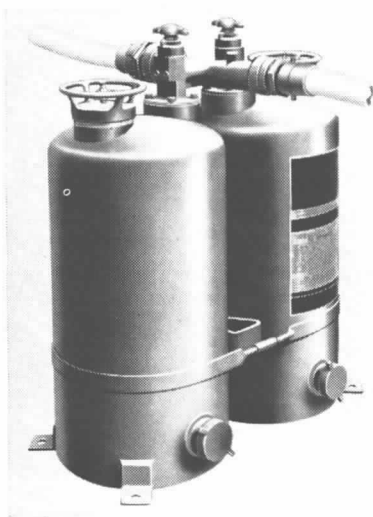
Pressure Proportioner, Dual Tank.
