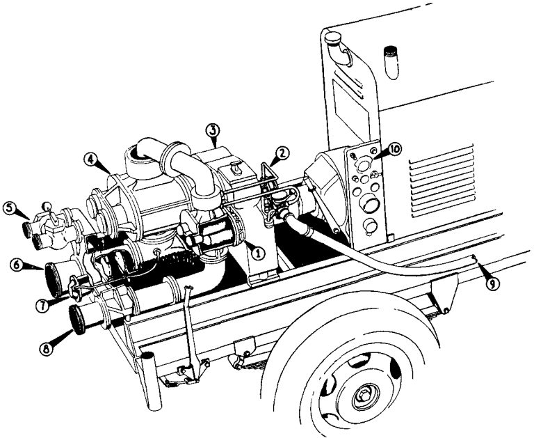
Fig. A-1154. Air Foam Pump.
