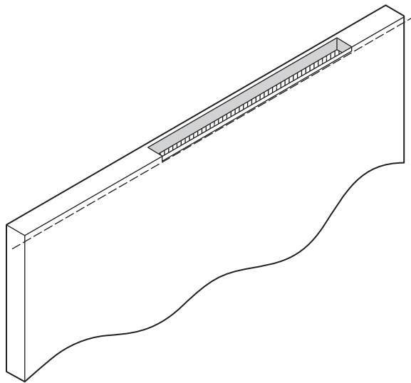
FIGURE A.6.7.1.2 Mortise Cutout in Top of Door Leaf for Overhead Door Stop. The dotted line represents the height of the door stop on the door frame. Gasketing should be installed on the soffit of the door frame so that it contacts the surface of the door below the cutout.
