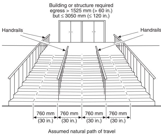
FIGURE A.5.2.2.4.2 Assumed Natural Paths of Travel on Monumental Stairs with Various Handrail Locations.
