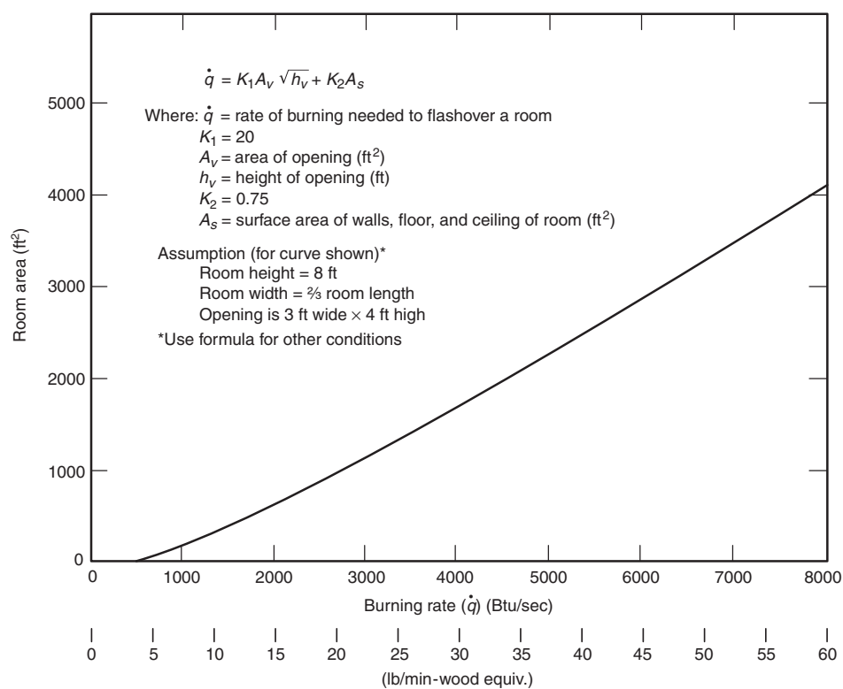
FIGURE 8.5.2.1(B) Approximate Flashover Energy.
