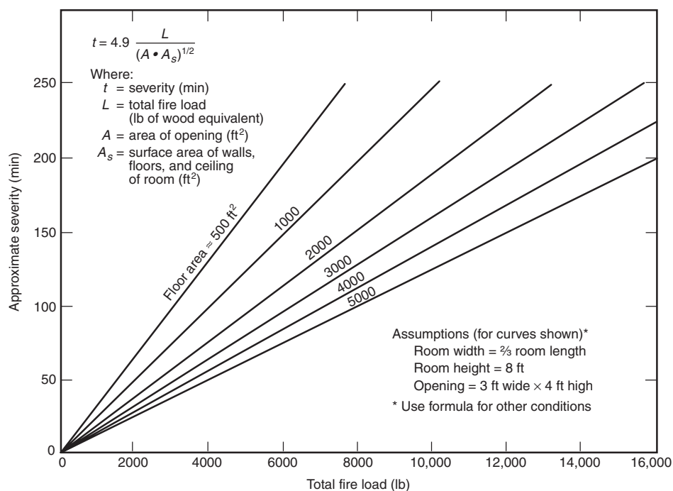
FIGURE 8.5.2.1(A) Approximate Fire Severity.
