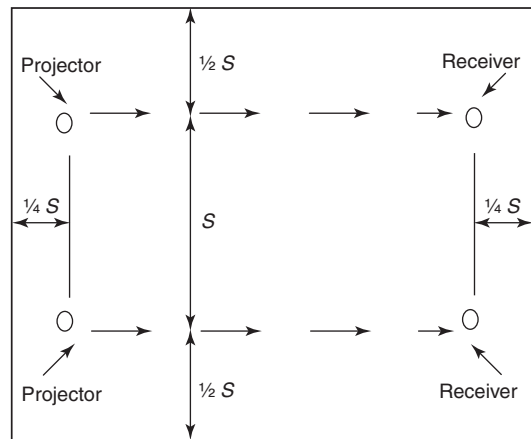
FIGURE A.13.7.4.3.5 Maximum Distance at Which Ceiling-Suspended Light Projector and Receiver Can Be Positioned from End Wall Is One-Quarter Selected Spacing ( S ). [72: A.5.7.3.4]
