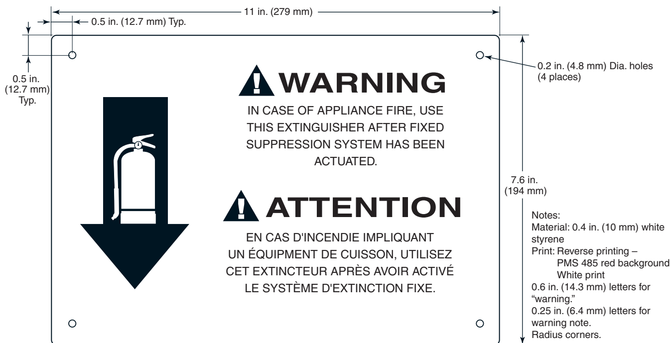
FIGURE A.13.6.7.4.5.3(b) Typical Class K Placard (English/French). [10: Figure A.5.5.3(b)]
