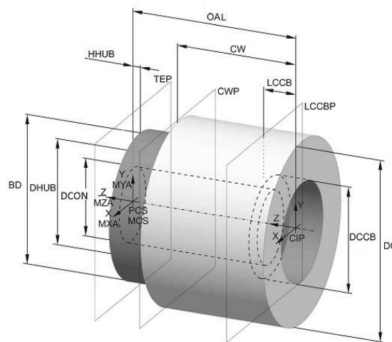
Figure 13 — Shell mill, complete
