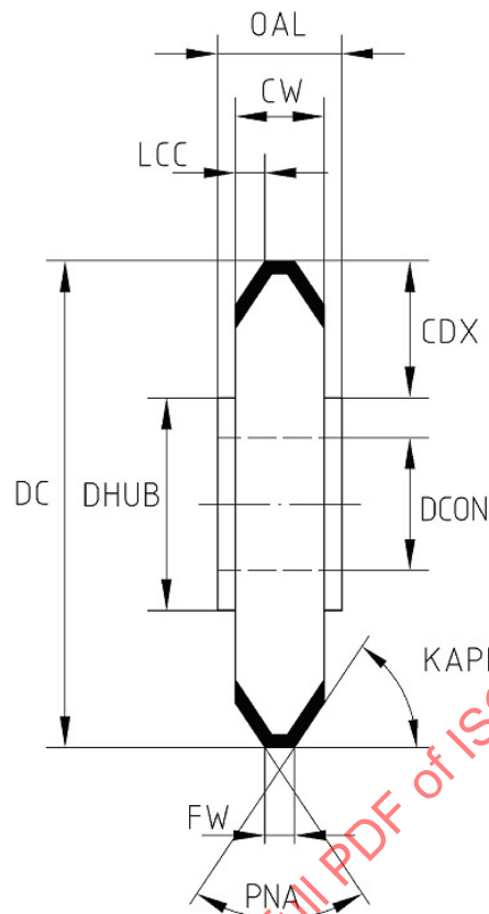
Figure 20 — Flatted profile slotting cutter: Determination of properties
