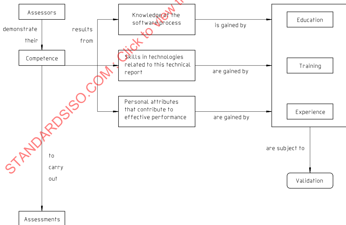
Figure 1 — Entity relationships
