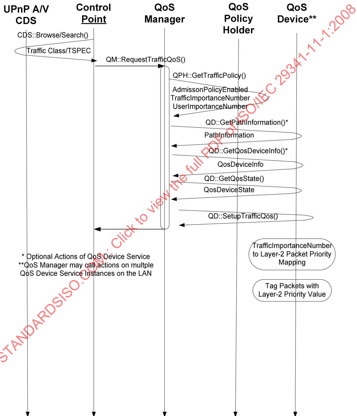
Figure 3 – Packet Priority Determination Flow
