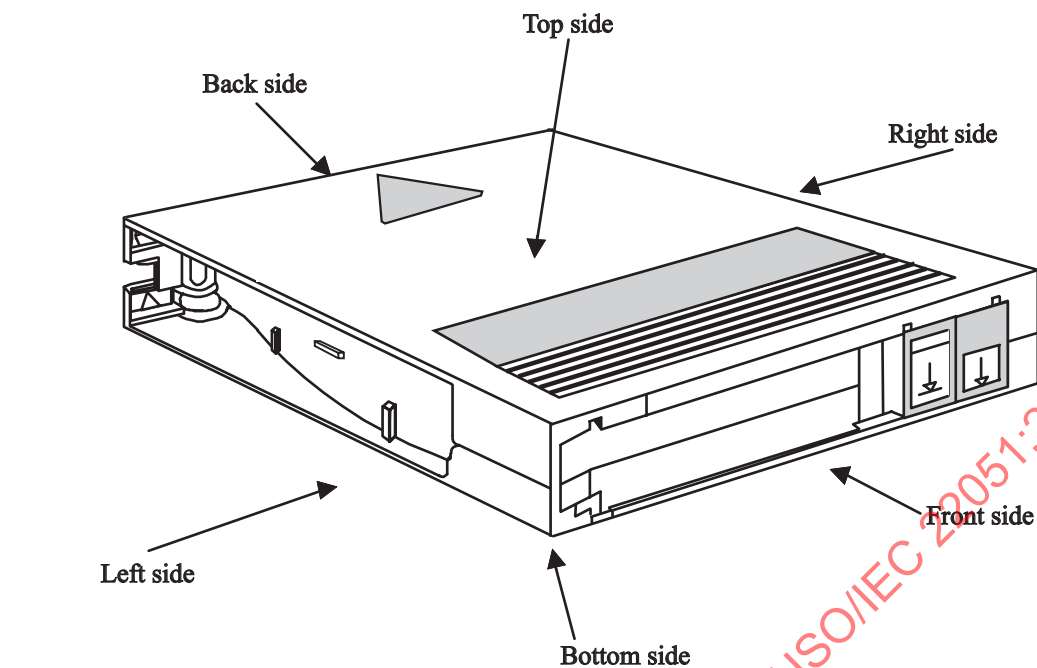
Figure 6 - General view
