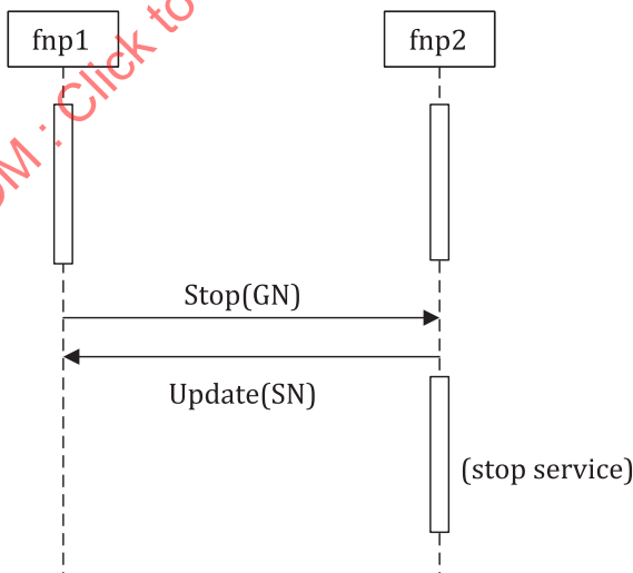
Figure 7 — Procedure of stopping FNProxy service
