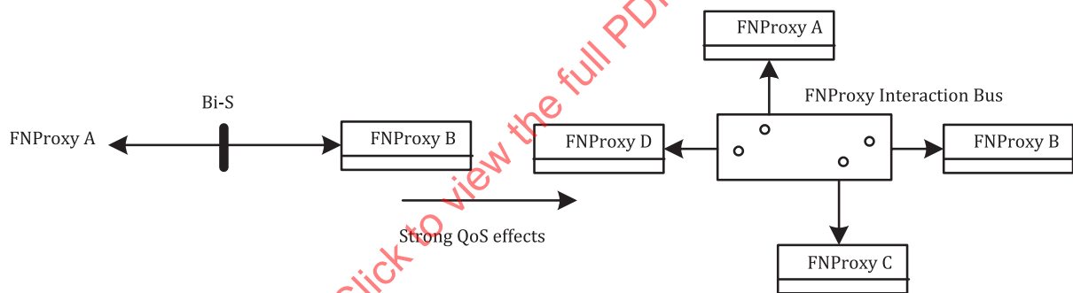
Figure 9 — Synthetic FNQoS system (SFS) with FIB
