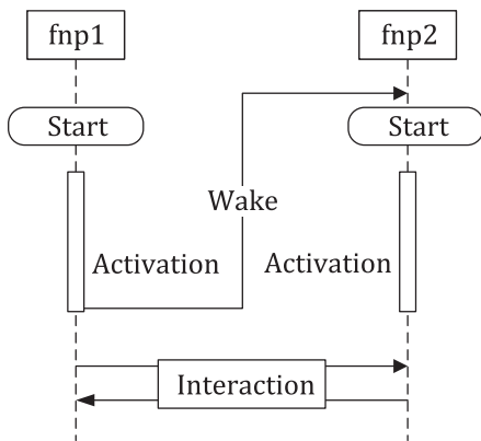
Figure 6 — Waking up the other party's procedure
