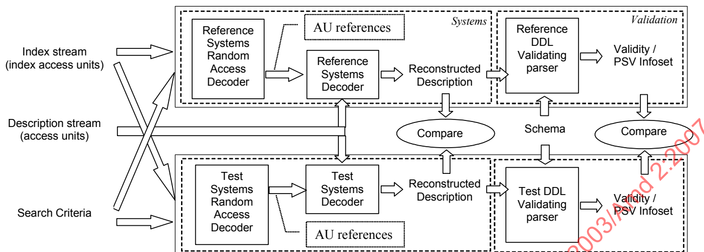
Figure Amd2.2 — Overview of conformance testing of random access systems based validating terminals
