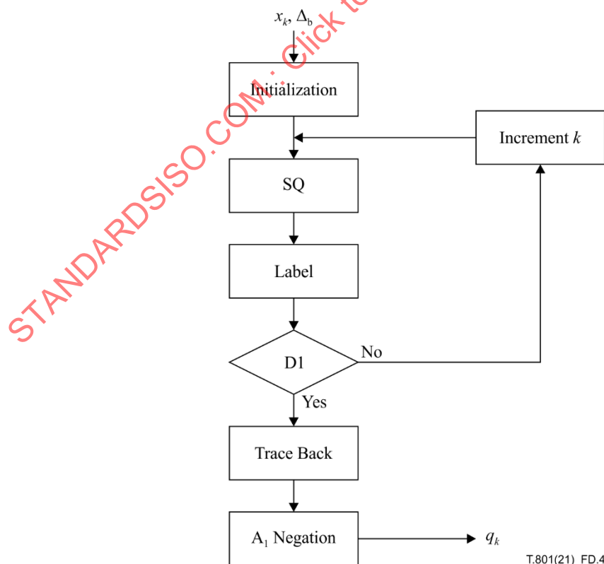
Figure D.4 – Forward TCQ processing
