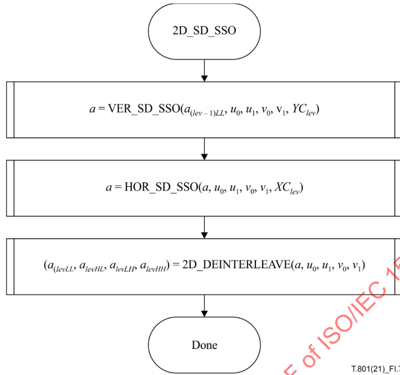
Figure I.7 – The 2D_SD_SSO procedure
