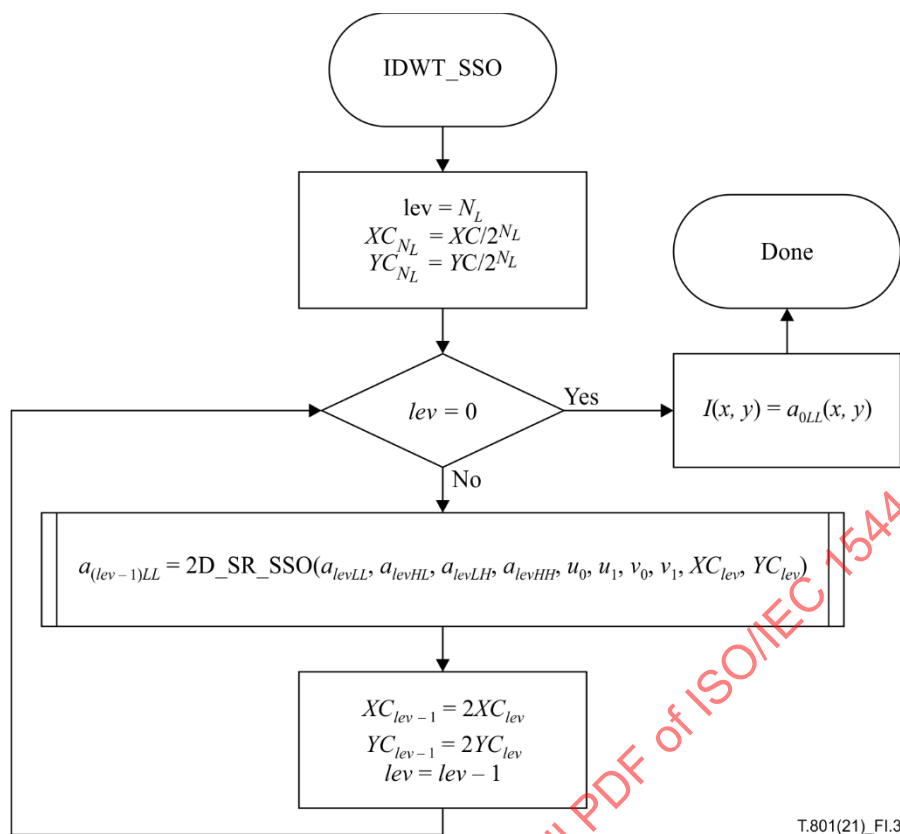
Figure I.3 – The IDWT_SSO Procedure
