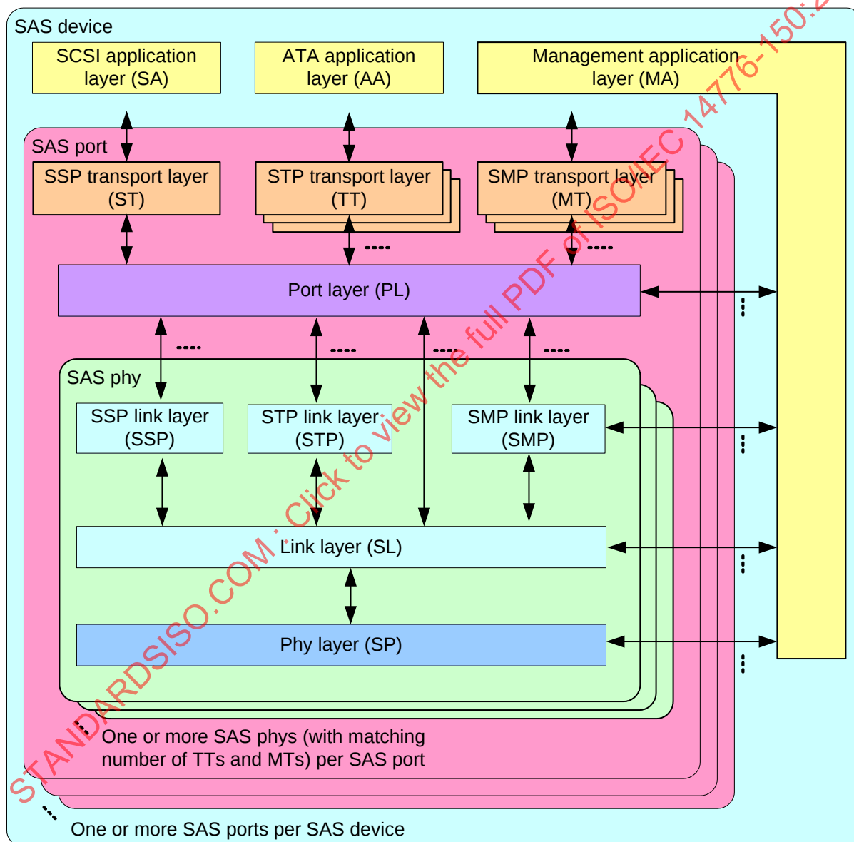
Figure 23 — State machines for SAS devices
