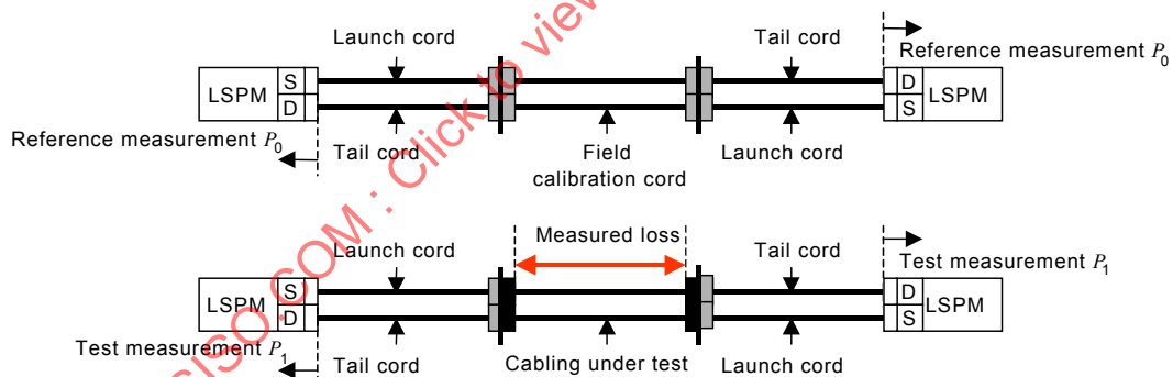
Figure 9 – LSPM 3-jumper attenuation measurement of installed cabling
