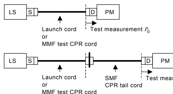
Figure A.4 – CPR measurement method
