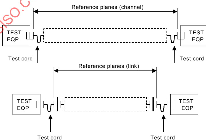
Figure 8 – Channel and permanent link test configuration
