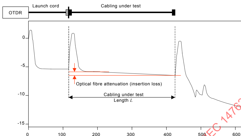
Figure 13 – OTDR measurement of optical fibre attenuation
