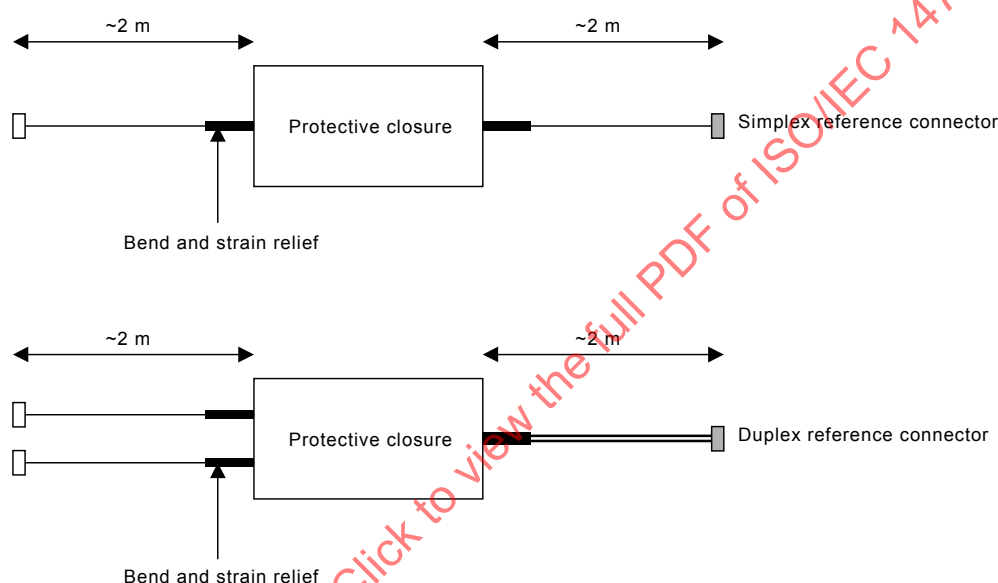
Figure 6 – OTDR launch cord schematic
