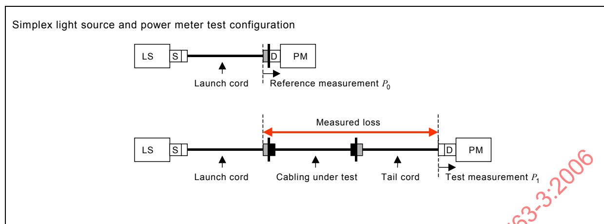
Figure 10 – LSPM 1-jumper attenuation measurement of installed link
