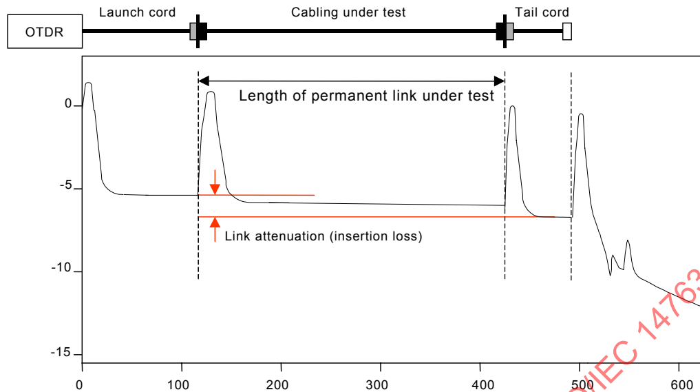
Figure 11 – OTDR measurement of installed cabling (permanent link)
