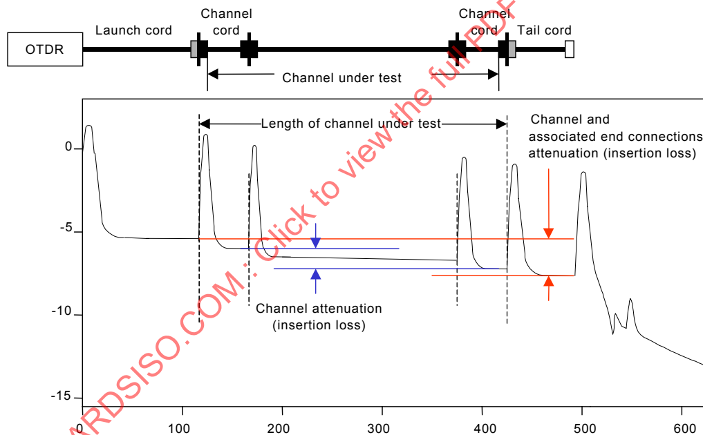
Figure 12 – OTDR measurement of installed cabling (channel)
