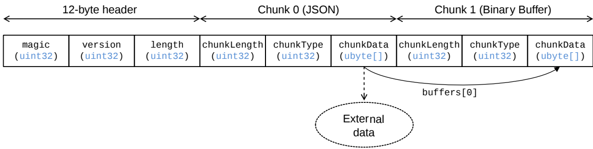
Figure 8. Binary glTF Layout
