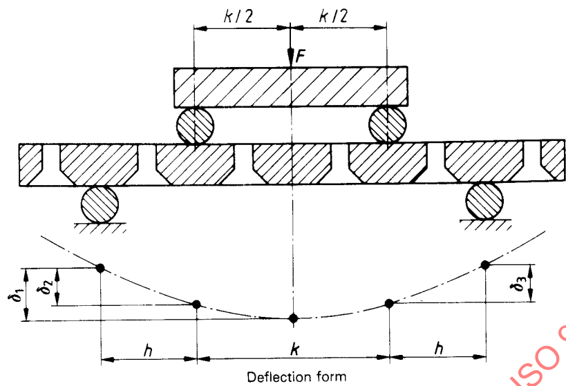
Figure 1 — General arrangement of four-point bend test
