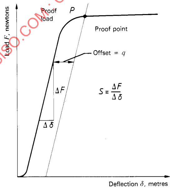
Figure 2 — Load deflection diagram
