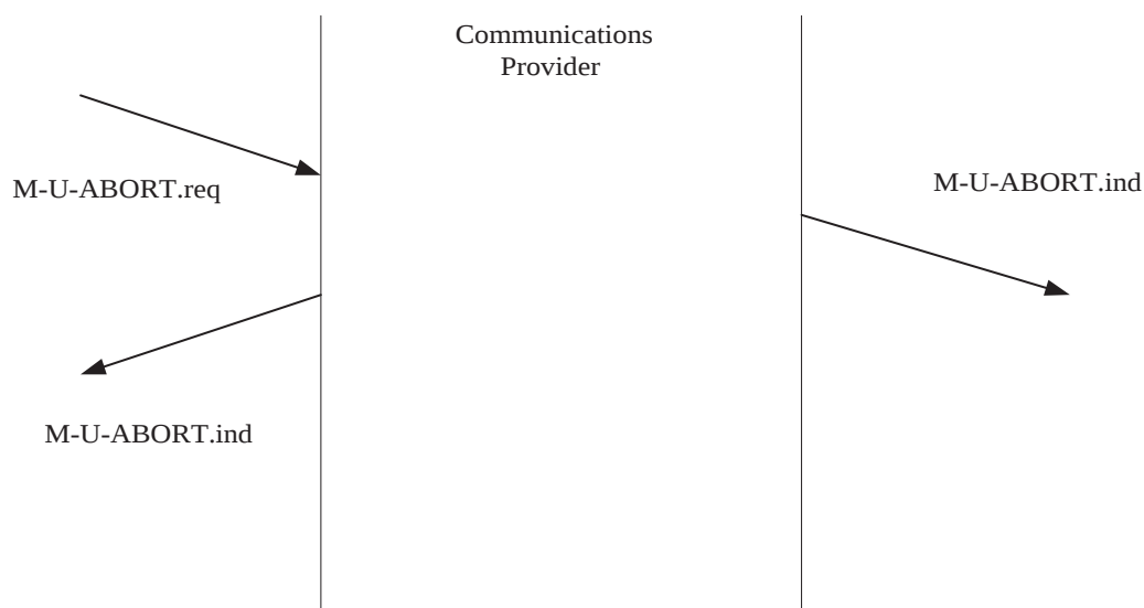
Figure 5 - M-U-ABORT service
