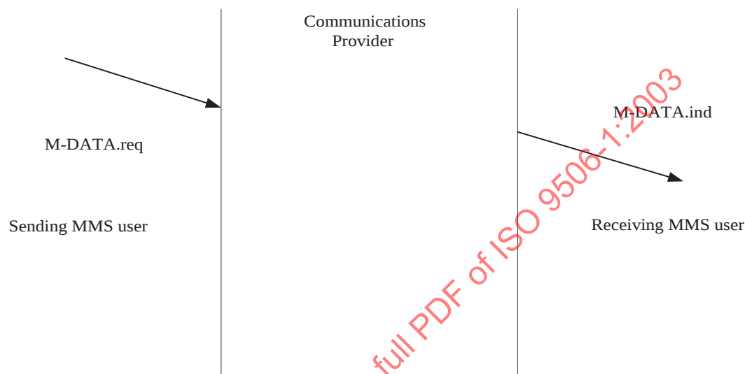
Figure 4 - M-DATA service
