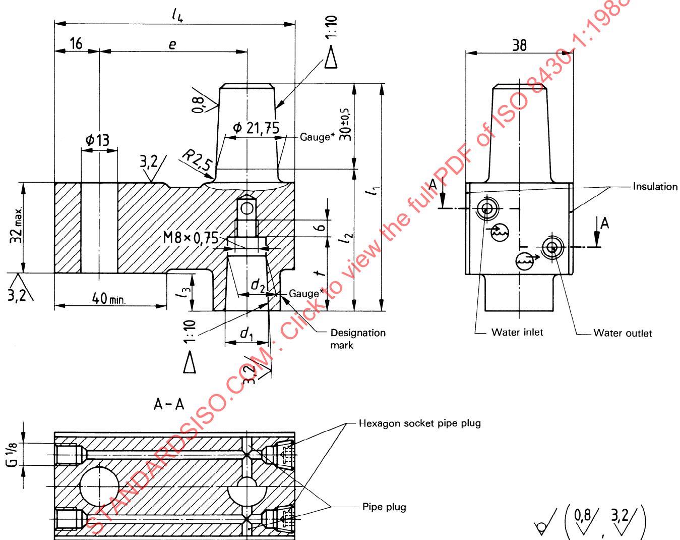
Figure 1 — Dimensions
