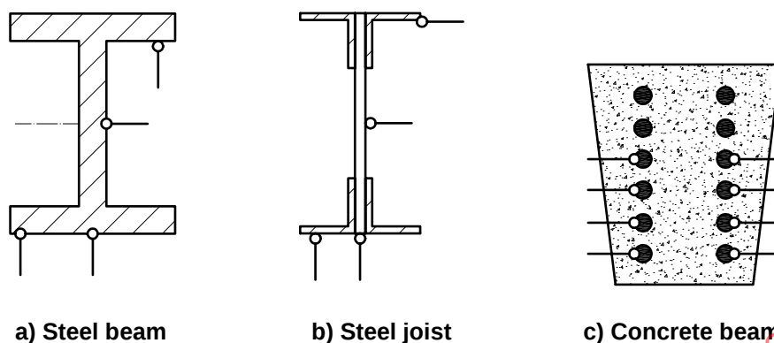
Figure 2 — Typical positions for specimen thermocouples
