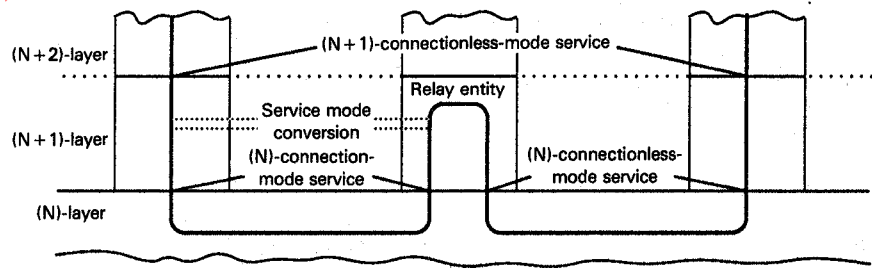
d) Connection- and connectionless-mode services yielding a connectionless-mode service
