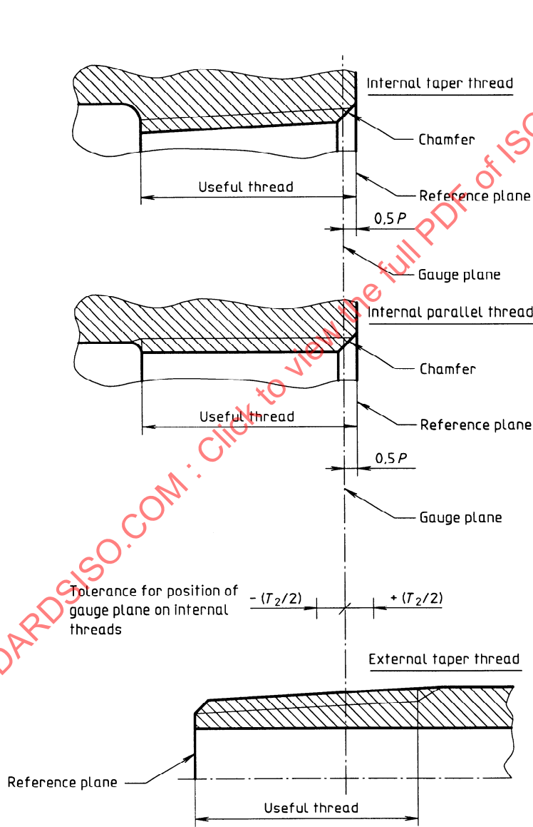
Figure 5 — Illustration of internal and external pipe threads (position of gauge plane, reference plane useful thread)
