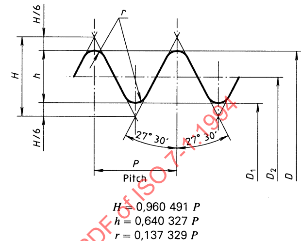
Figure 1 — Parallel thread
