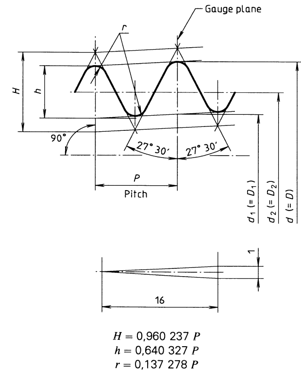
Figure 2 — Taper thread
