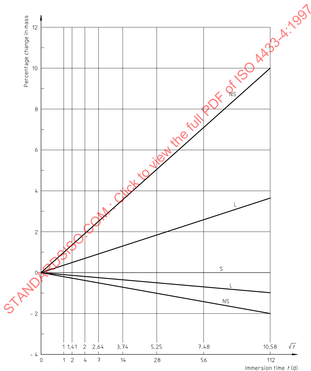
Figure 1 — Classification diagram for PVDF pipes based on change in mass
