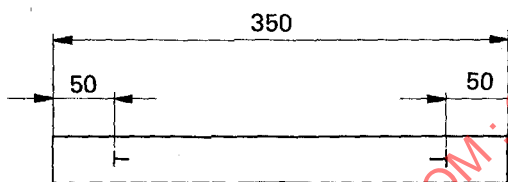
Marking of specimen for fabric of width less than 650 mm
