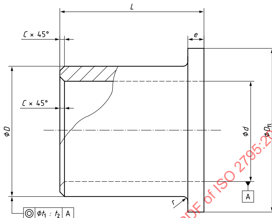
Figure 2 — Flanged bearing
