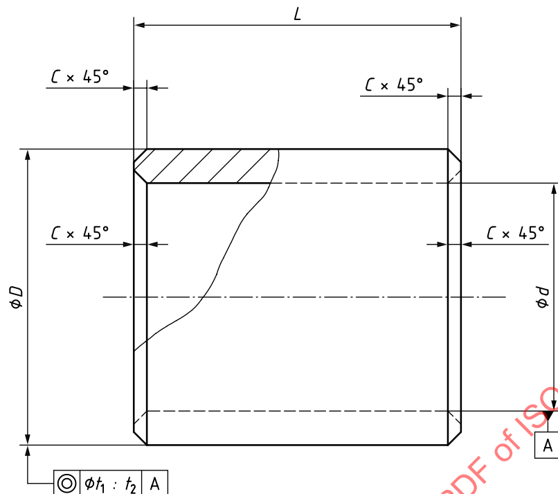
Figure 1 — Cylindrical bearing
