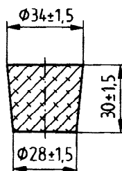
Figure 5 — Stopper
