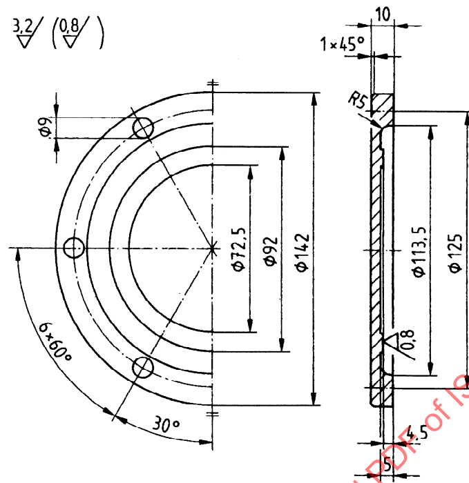
Figure 3 — Flange plate
